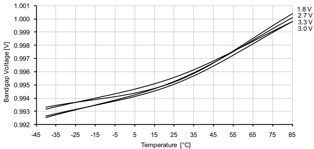
Figure 33-214. ADC Internal 1.0V reference vs. temperature.
