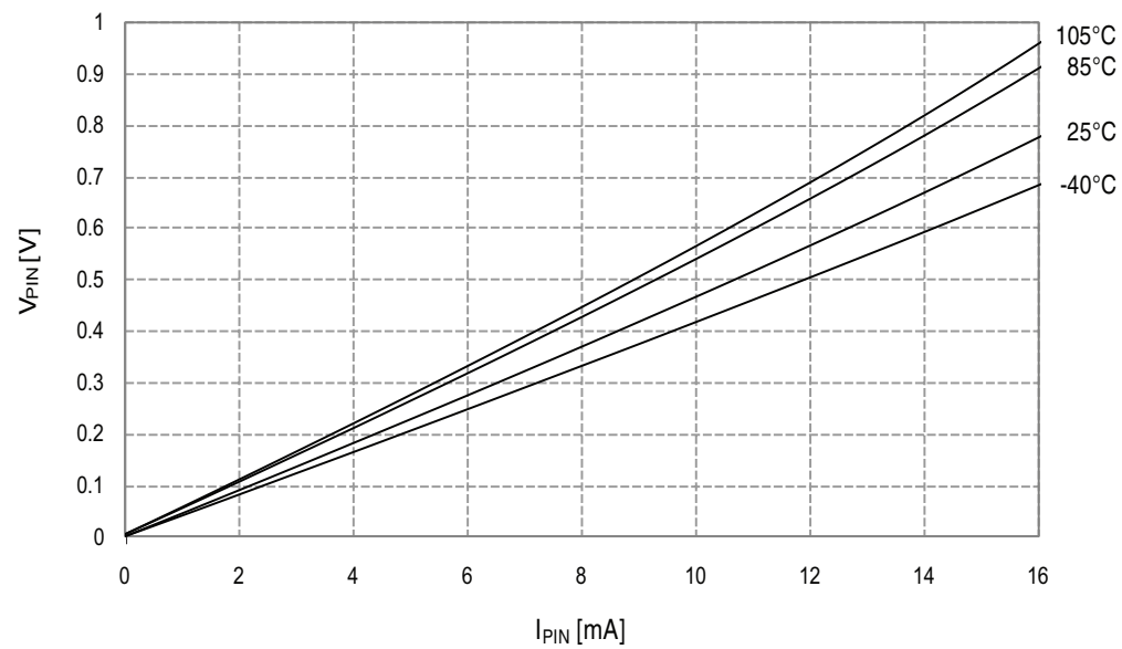
Figure 33-109. I/O pin output voltage vs. sink current.
