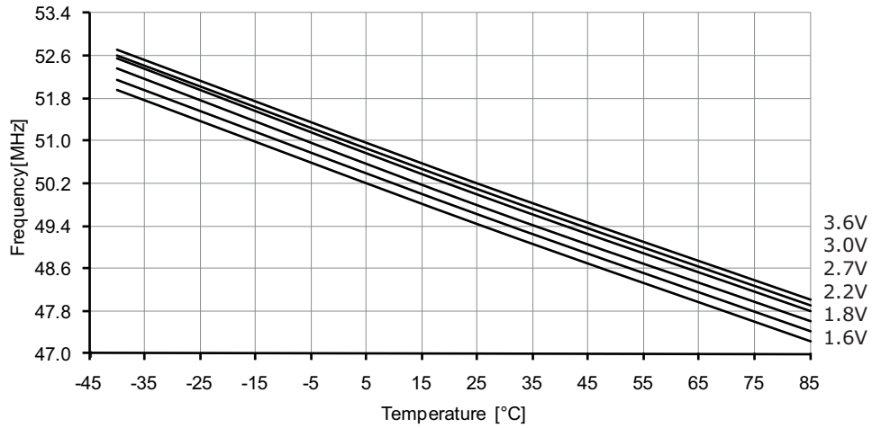
Figure 33-236. 48MHz internal oscillator frequency vs. temperature. DFLL enabled, from the 32.768kHz internal oscillator.
