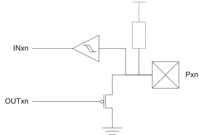
Figure 14-6. I/O configuration - Wired-AND with optional pull-up.
