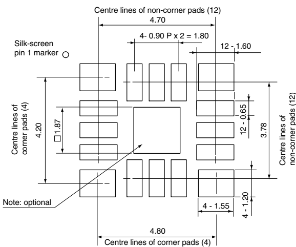
Figure 7.2 Recommended Pad Layout (CRM102.1)
