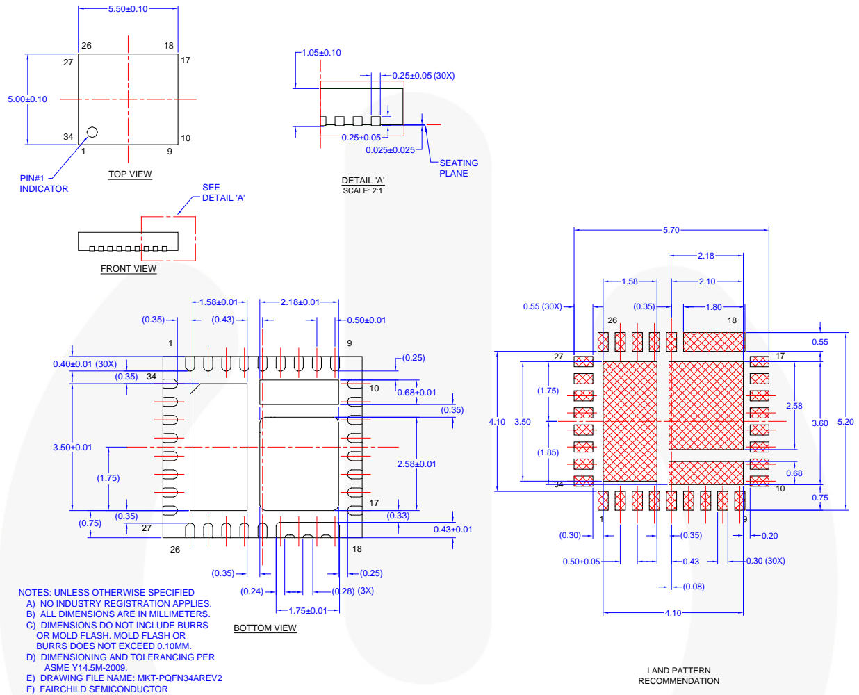
Figure 34. 34-Lead, PQFN, 5.5 mm x 5.0 mm
