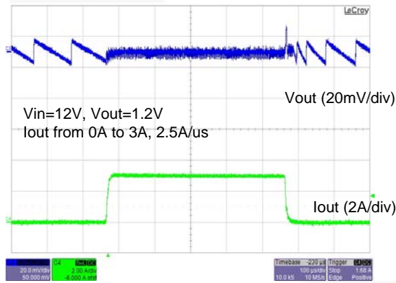
Figure 27. FAN2306M Load Transient from 0% to 50% Load Current
