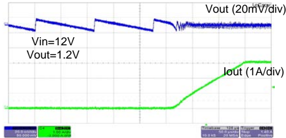
Figure 17. FAN2306M Transition from DCM to CCM
