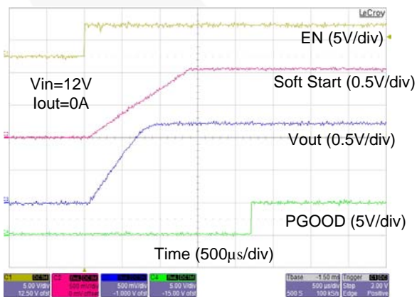
Figure 15. Startup Waveforms with 0 A Load Current
