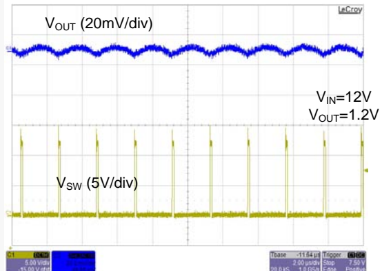
Figure 15. Static Output Ripple with No Load
