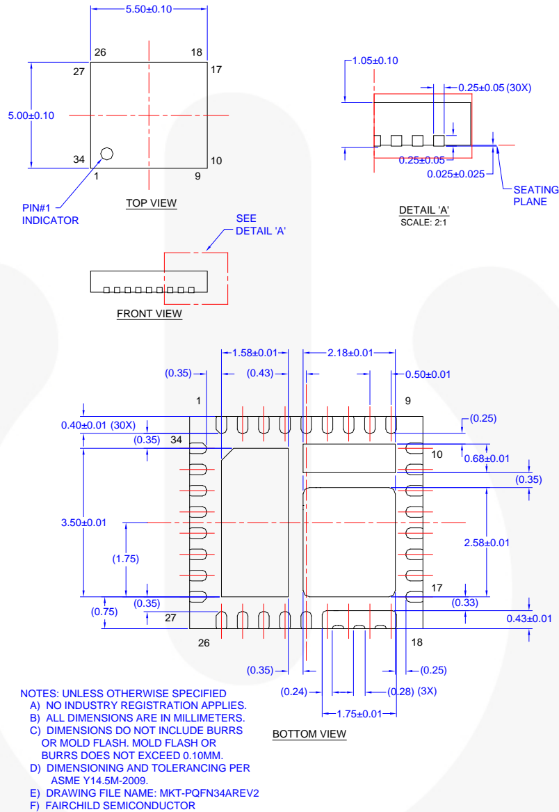
Figure 26. 34-Lead, PQFN, 5.5 mm x 5.0 mm
