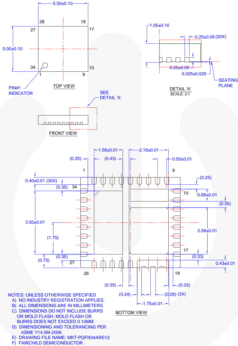
Figure 34.34-Lead, PQFN, 5.5 mm x 5.0 mm Package
