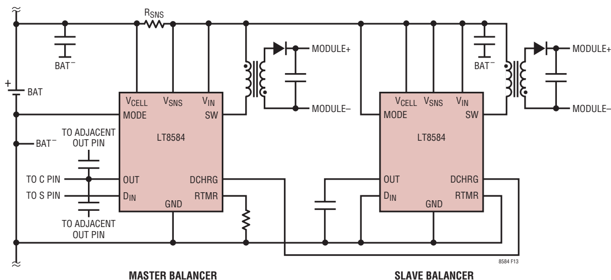
Figure 13. LT8584 Parallel Operation
