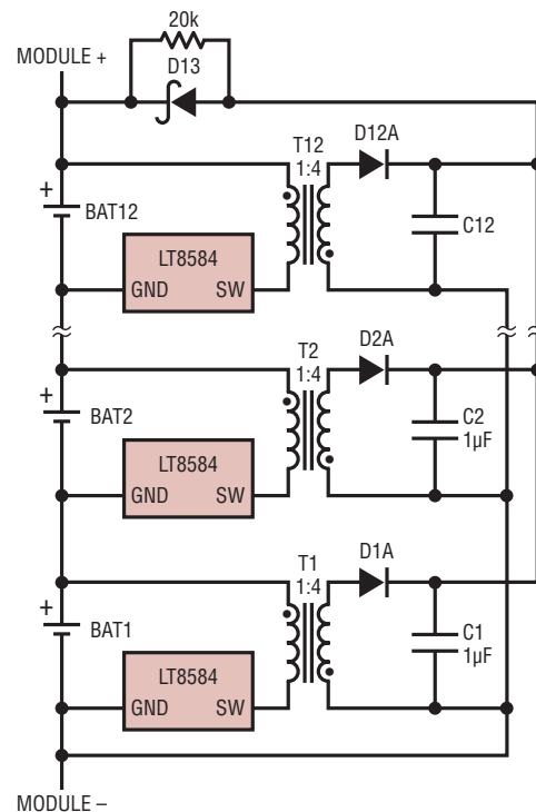
Figure 12. Active Hot Swap Solutions
