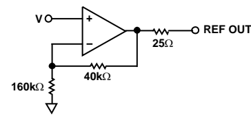
Figure 18. AD7495 Reference Circuit
