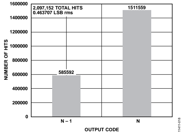
Figure 18. Grounded Input Histogram
