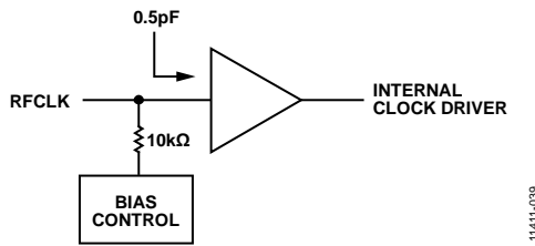
Figure 39. Equivalent RF Clock Input Circuit
