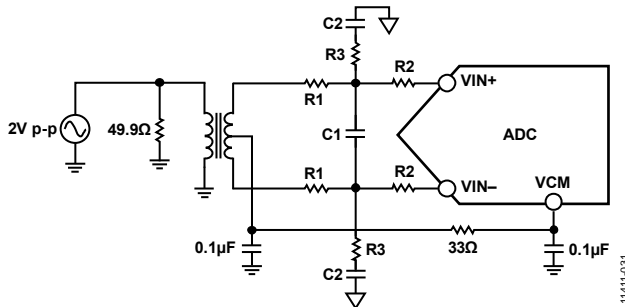
Figure 31. Differential Transformer-Coupled Configuration
