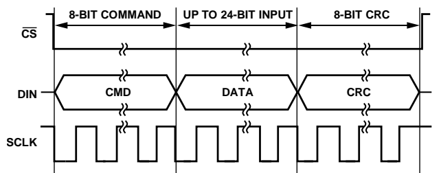
Figure 72. SPI Write Transaction with CRC
