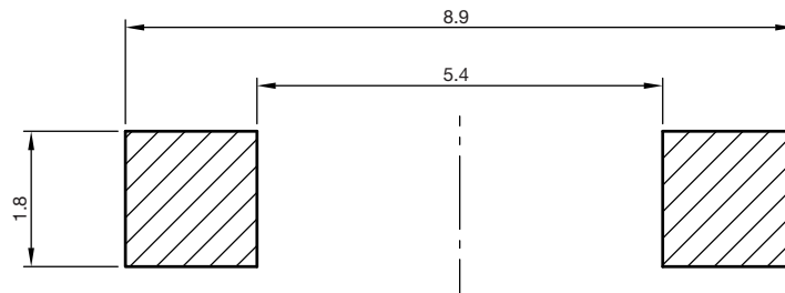
Recommended solder pad
