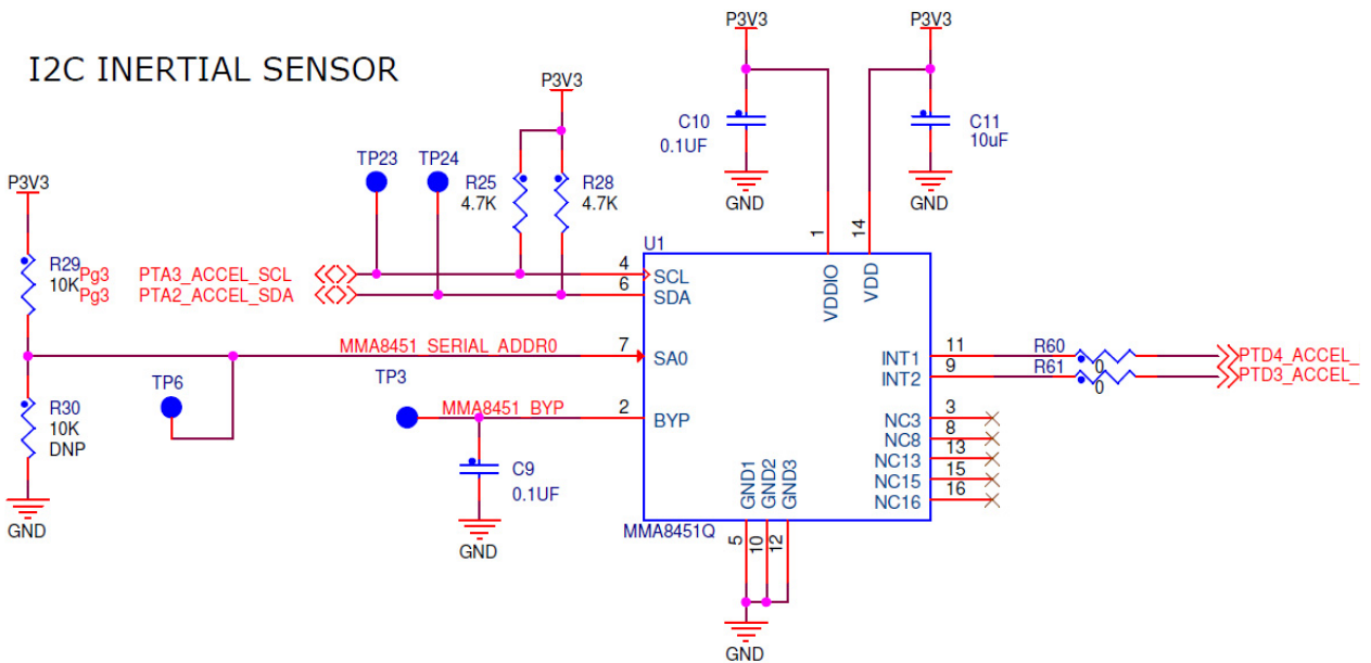
Figure 8. Accelerometer connection
