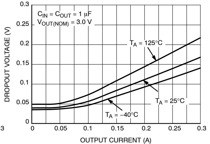
Figure 21. Dropout Voltage vs. Output Current V_{OUT} = 3.0\text{ V}
