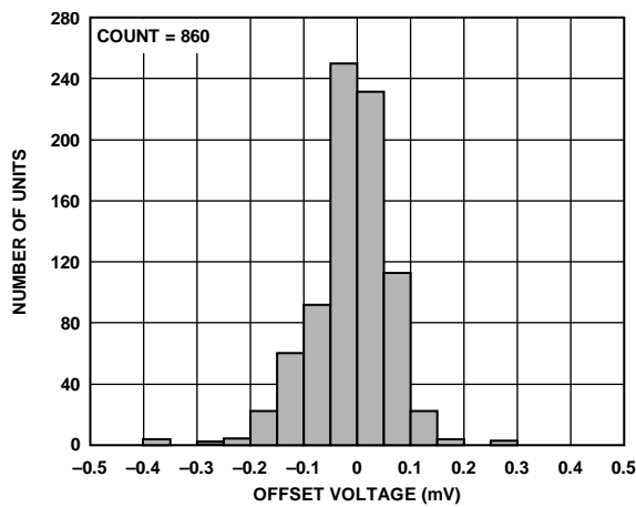
Figure 14. Input Offset Distribution, V_S = 5\text{V}, 0\text{V}
