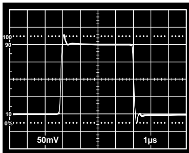
Figure 8. Open-Loop Gain/Phase and Small Signal Response, V_S = 3\text{ V} , C_L = 220\text{ pF}
