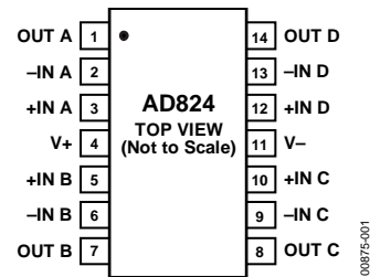
Figure 1. 14-Lead Epoxy SOIC (R Suffix)
