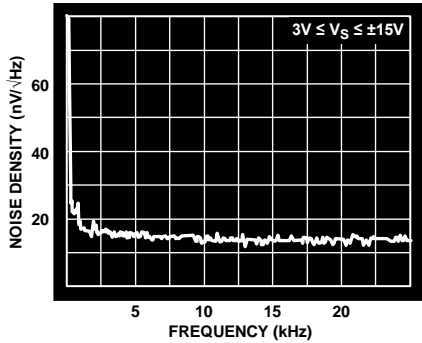
Figure 12. Voltage Noise Density
