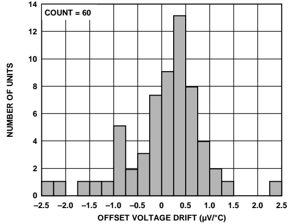
Figure 15. TC V_{0S} Distribution, -55^{\circ}\text{C} to +125^{\circ}\text{C} , V_S = 5\text{V}, 0\text{V}
