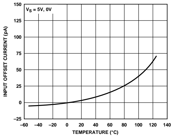
Figure 16. Input Offset Current vs. Temperature
