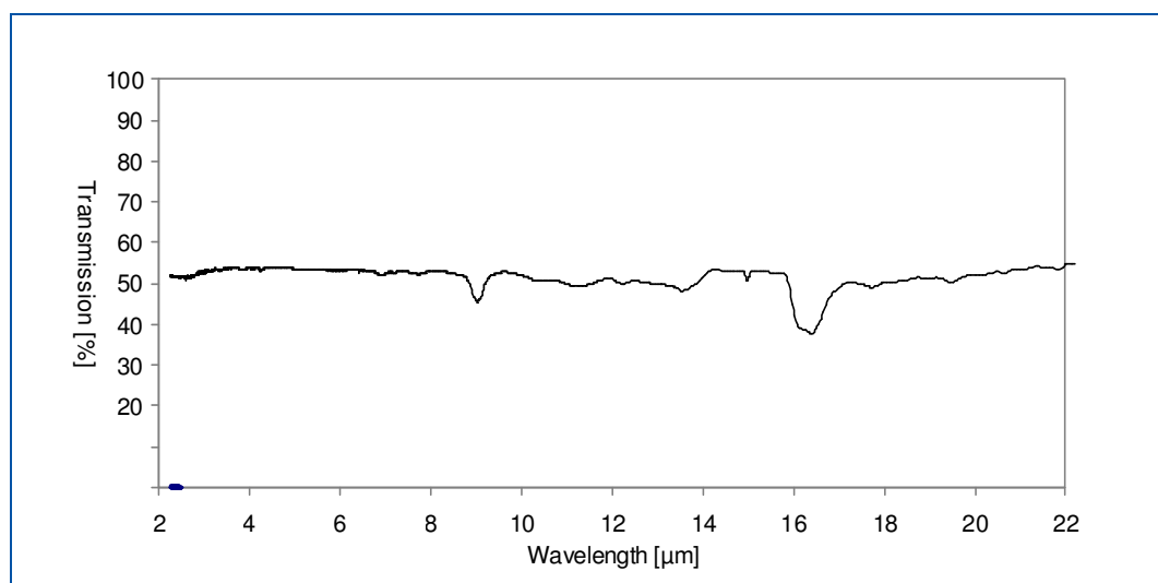
Figure 3: IR-Filter characteristic
