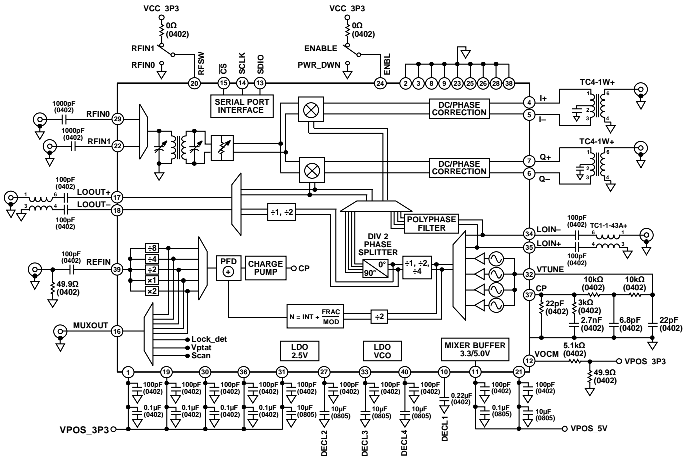
Figure 33. Basic Connections
