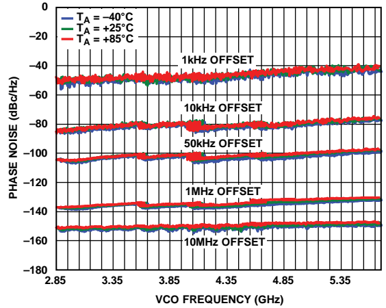
Figure 18. Open-Loop Phase Noise for 1 kHz, 10 kHz, 50 kHz, 1 MHz, and 10 MHz Offsets
