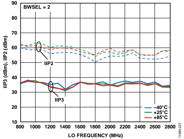
Figure 8. Input IP3 (IIP3) and Input IP2 (IIP2) vs. LO Frequency over Temperature, BWSEL = 2
