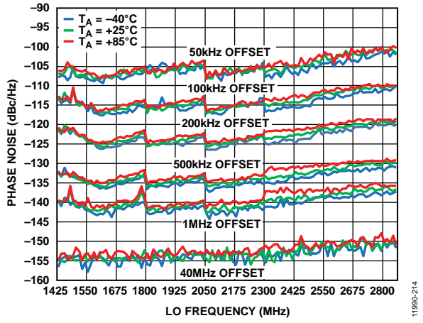
Figure 20. Closed-Loop Phase Noise vs. LO Frequency, 20 kHz Bandwidth Loop Filter, Measured with DIV4\_EN = 1 (Divide by 2)
