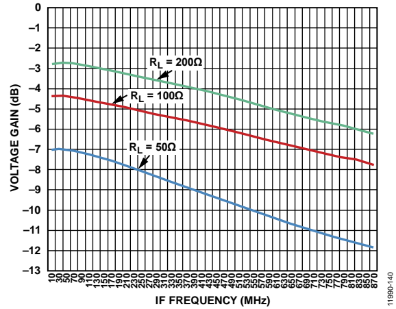
Figure 47. Voltage Gain vs. IF Frequency for f_{LO} = 1840 \text{ MHz} , BWSEL = 2
