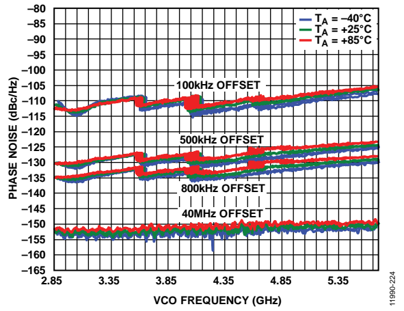
Figure 19. Open-Loop Phase Noise for 100 kHz, 500 kHz, 800 kHz, and 40 MHz Offsets
