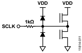
Figure 22. Equivalent SCLK Circuit
