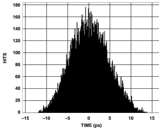
Figure 41. Time Interval Histogram Error of JESD204B Output at 6.25 Gbps
