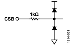
Figure 25. Equivalent CSB Input Circuit
