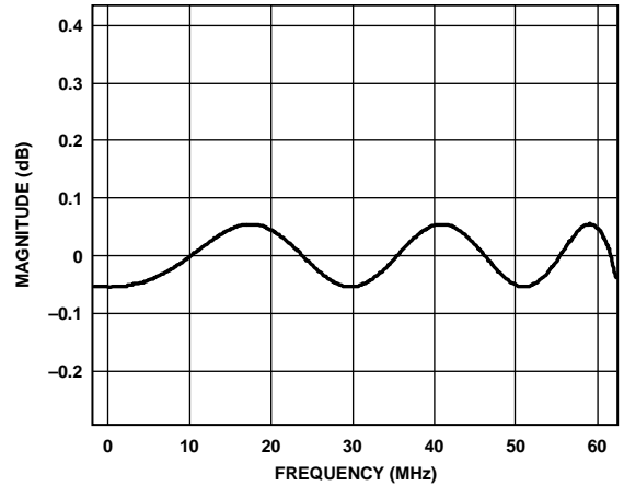
Figure 32. Magnitude Ripple in the Pass Band
