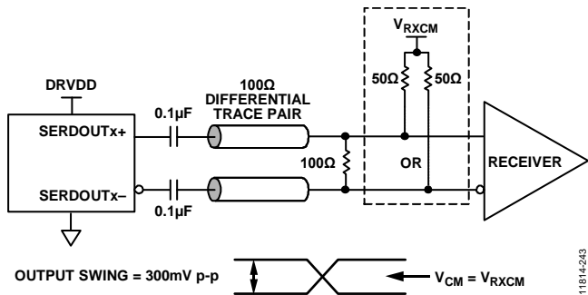
Figure 37. DC-Coupled Digital Output Termination Example
