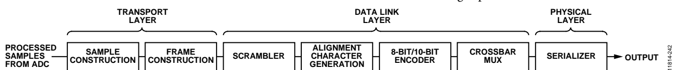
Figure 35. Data Flow
