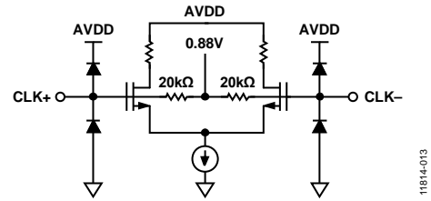
Figure 24. Equivalent Clock Input Circuit
