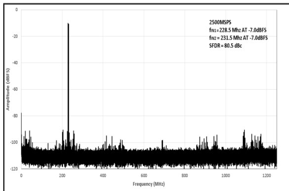
Figure 18. Two Tone FFT Plot at 2.5 GSps, f_{IN1} = 228.5 MHz and f_{IN2} = 231.5 MHz at AIN, -7 dBFS (SFDR = 80 dBc)
