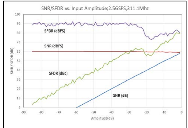
Figure 8. SNR/SFDR vs. Analog Input Amplitude at 2.5GSPS, f_{IN} = 311.1 MHz at AIN
