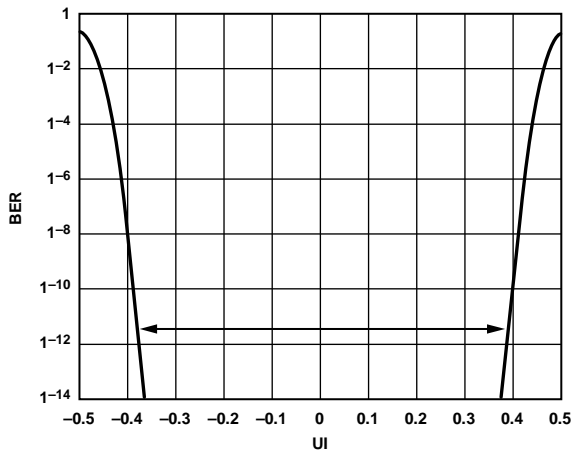
Figure 40. Bathtub Plot of JESD204B Output at 6.25 Gbps
