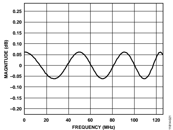
Figure 30. Magnitude Ripple in the Pass Band
