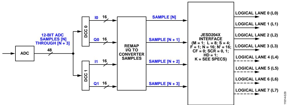
Figure 42. DDC Mapping
