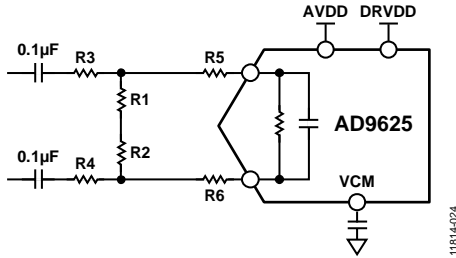
Figure 33. Front-End Minimum Requirement
