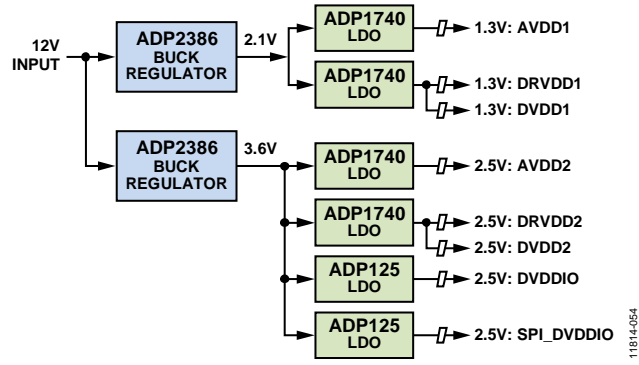
Figure 45. Power Supply Recommendation
