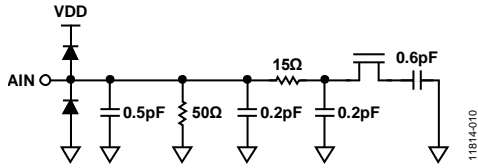
Figure 21. Equivalent Analog Input Circuit
