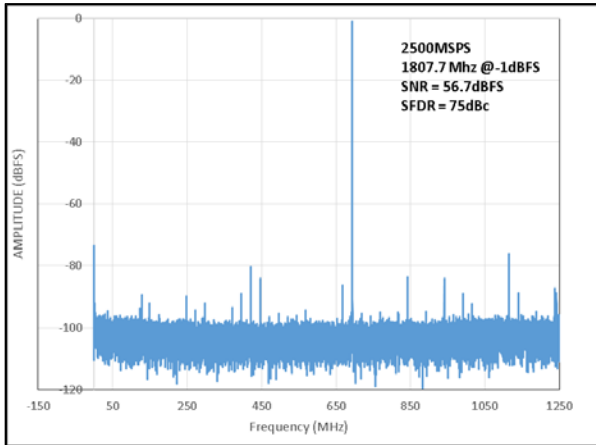
Figure 5. FFT Plot at 2.5 GSPS, f_{IN} = 1807.7 MHz at AIN (SFDR = 75.0 dBc, SNR = 56.7 dBFS)
