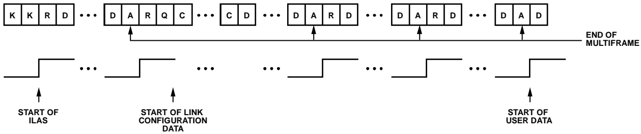
Figure 38. Initial Lane Alignment Sequence
