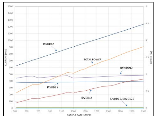
Figure 10. Current and Power vs. Sample Rate
