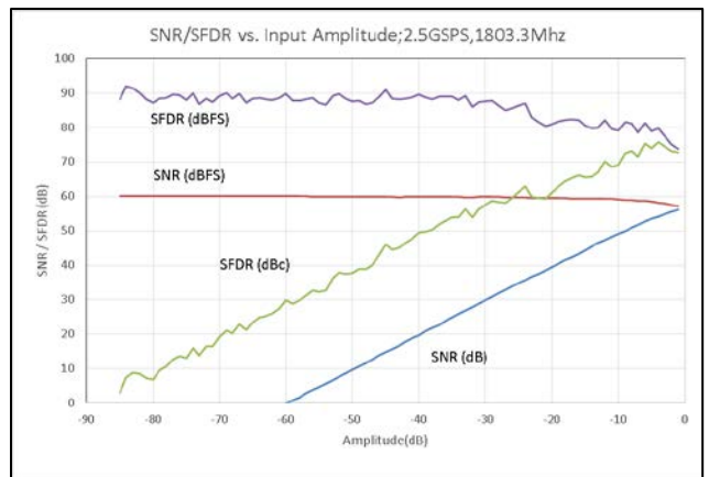
Figure 9. SNR/SFDR vs. Analog Input Amplitude at 2.5 GSPS, f_{IN} = 1803.3 MHz at AIN
