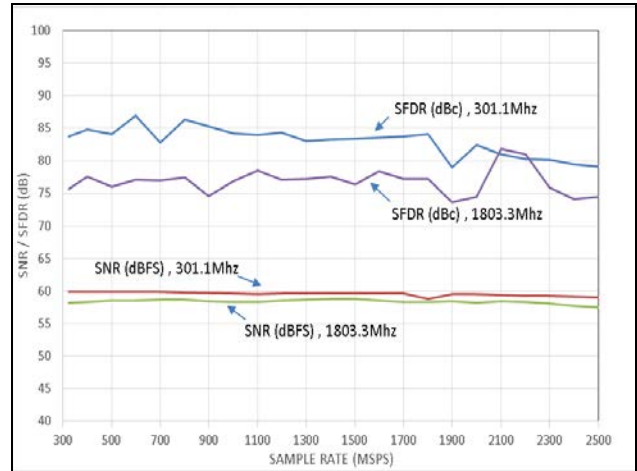
Figure 14. SNR/SFDR vs. Sample Rate
