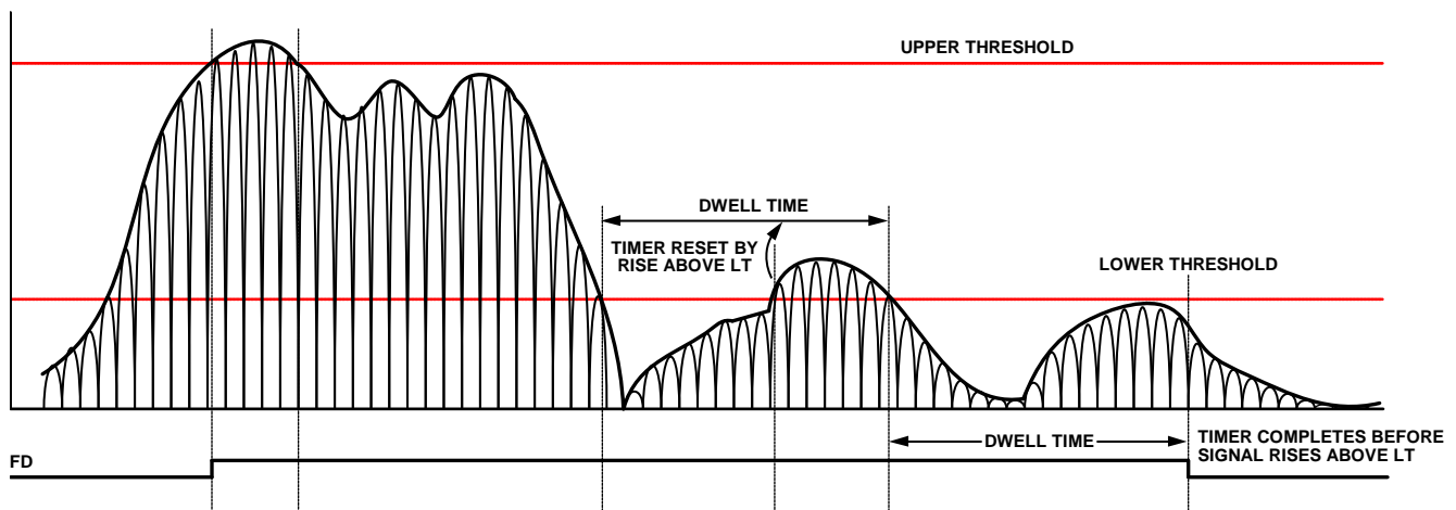
Figure 27. Fast Detection Bit
