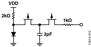
Figure 23. Equivalent Temperature Sensor Circuit
