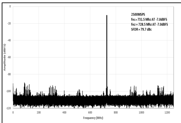
Figure 17. Two Tone FFT Plot at 2.5 GSps, f_{IN1} = 728.5 MHz and f_{IN2} = 731.5 MHz at AIN, -7 dBFS (SFDR = 79.7 dBc)
