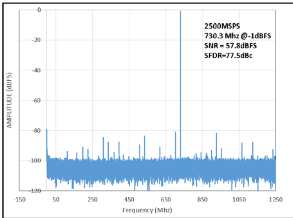
Figure 6. FFT Plot at 2.5 GSPS, f_{IN} = 730.3 MHz at AIN (SFDR = 77.5 dBc, SNR = 57.8 dBFS)
