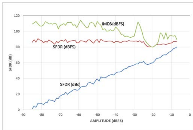
Figure 13. Two Tone SFDR and IMD3 vs. Analog Input Amplitude at 2.5 GSPS at 230 MHz AIN
