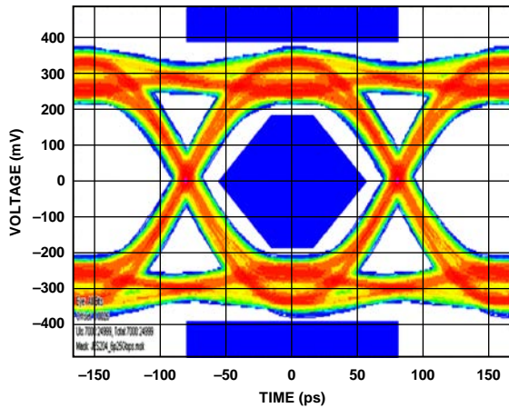
Figure 39. Recovered Data Eye of JESD204B Lane at 6.25 Gbps
