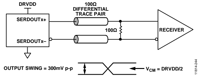
Figure 36. AC-Coupled Digital Output Termination Example
