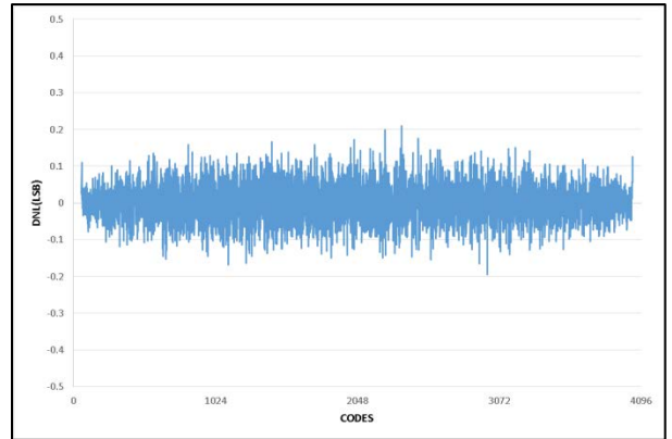
Figure 19. Differential Nonlinearity (DNL), \pm 0.2 LSB
