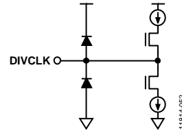
Figure 26. Equivalent DIVCLK± Output Circuit
