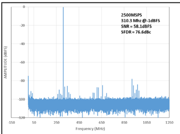
Figure 7. FFT Plot at 2.5 GSPS, f_{IN} = 310.13 MHz at AIN (SFDR = 76.6 dBc, SNR = 58.1 dBFS)
