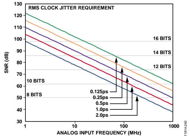
Figure 34. Ideal SNR vs. Analog Input Frequency and Jitter
