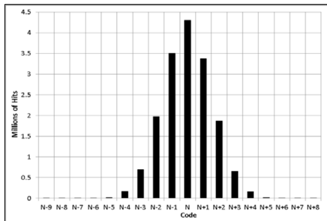
Figure 15. Input Referred Noise Histogram with 2.5Ghz Sample Clock
