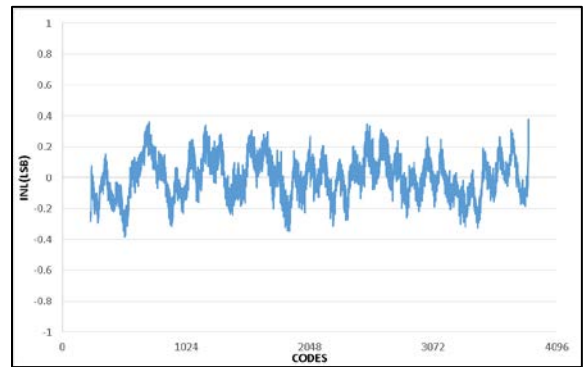
Figure 20. Integral Nonlinearity (INL), \pm 0.4 LSB
