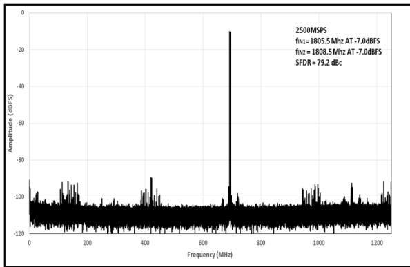
Figure 16. Two Tone FFT Plot at 2.5 GSps, f_{IN1} = 1805.5 MHz and f_{IN2} = 1808.5 MHz at AIN, -7 dBFS (SFDR = 79.2 dBc)
