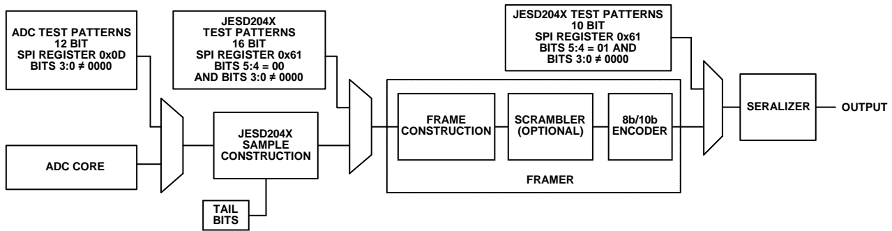
Figure 28. Test Modes
