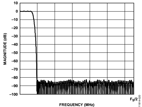
Figure 29. Magnitude Response of the Decimate-by-8 Polyphase Fuse Filter
