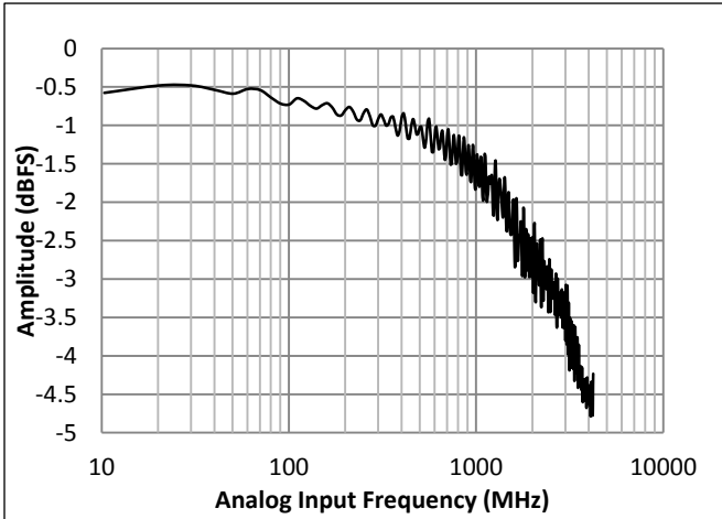
Figure 11. 3GHz Full Power Bandwidth at 2.5 GSPS
