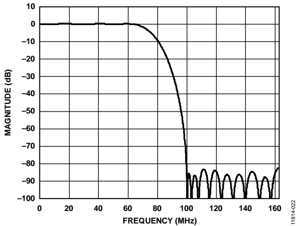
Figure 31. Magnitude Response of Decimate-by-2 Filter
