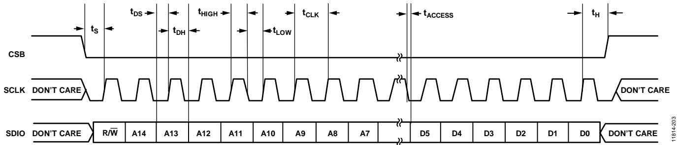
Figure 3. Serial Port Interface Timing Diagram (MSB First)
