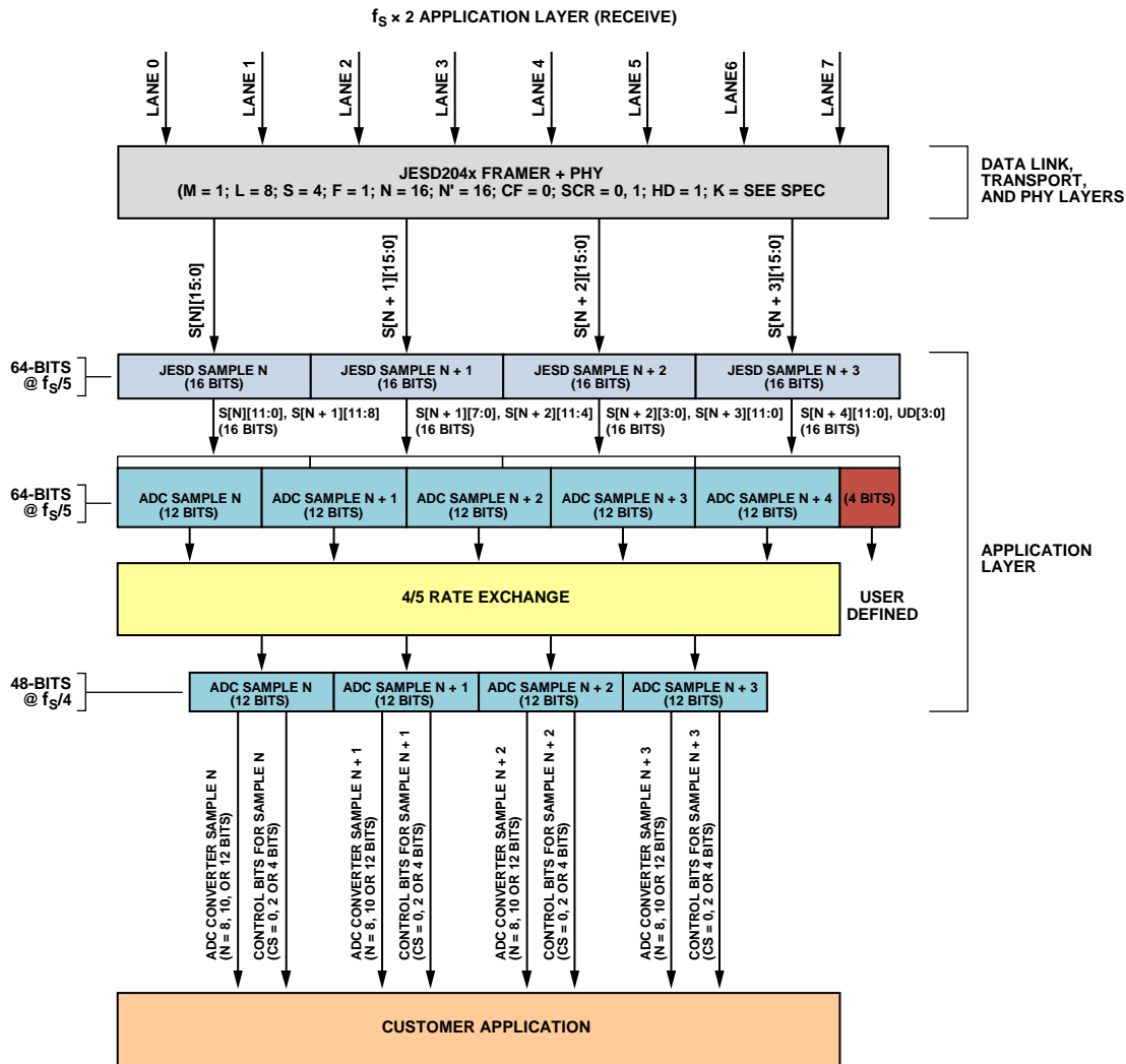
Figure 44. f_s \times 2 Application Layer (Receive)
