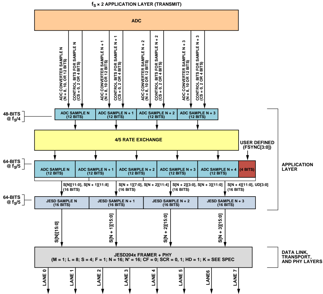
Figure 43. f_s \times 2 Mode Application Layer (Transmit)
