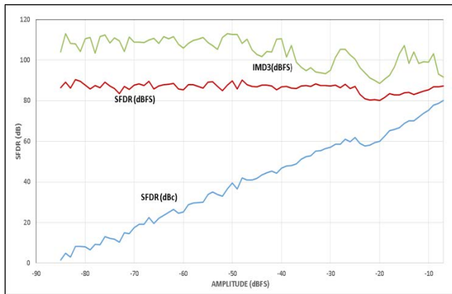
Figure 12. Two Tone SFDR and IMD3 vs. Analog Input Amplitude at 2.5GSPS at 1800 MHz AIN
