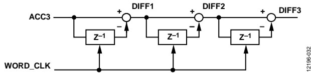
Figure 32. Differentiator
