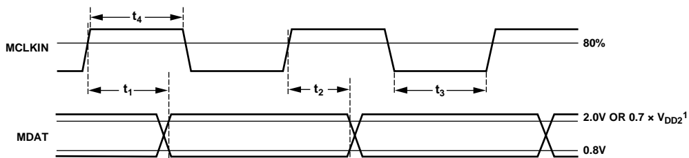
Figure 2. Data Timing
