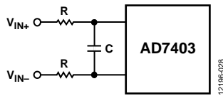
Figure 28. Differential RC Filter Network
