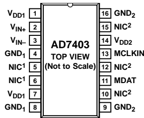
Figure 4. Pin Configuration
