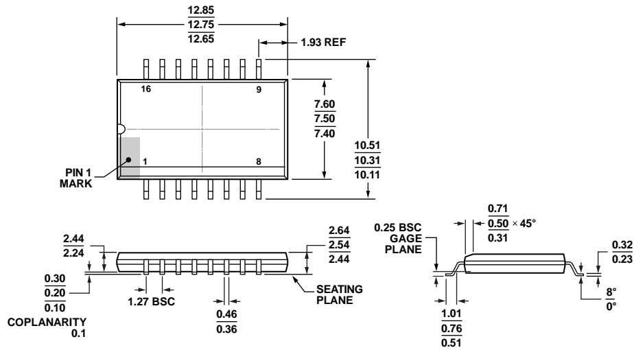
Figure 38. 16-Lead Standard Small Outline Package, with Increased Creepage [SOIC_IC] Wide Body (RI-16-2) Dimensions shown in millimeters
