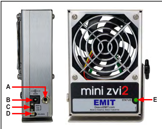
Figure 2. Mini Zero Volt Ionizer 2 features and components
