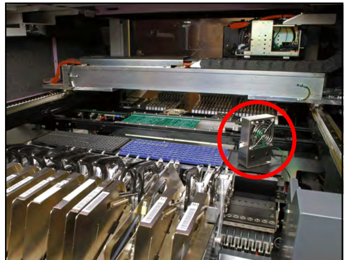
Figure 4. Using the Mini Zero Volt Ionizer 2 inside automated machinery.
