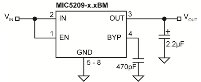
Figure 2. Ultra-Low-Noise Fixed Voltage Regulator
