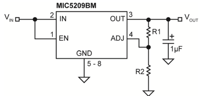
Figure 3. Low-Noise Adjustable Voltage Regulator
