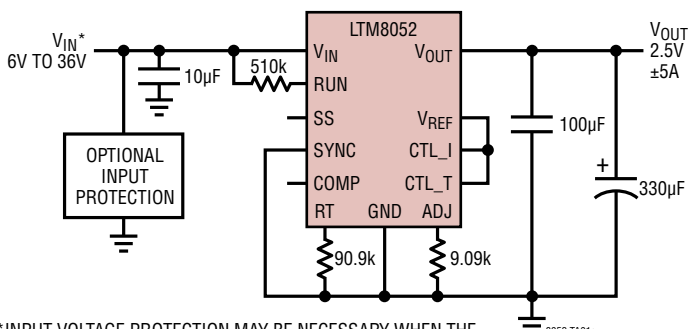
±5A, 2.5V (2-Quadrant) \mu Module Voltage Regulator
