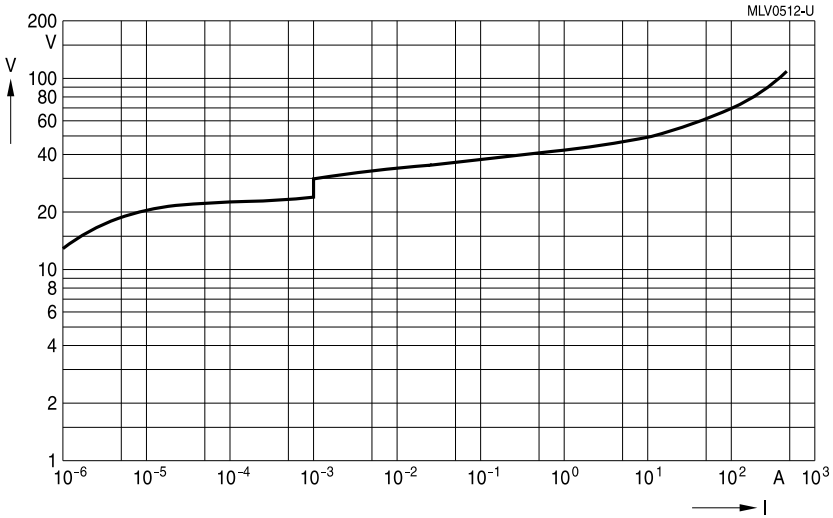
CT1210K17AUTOG
