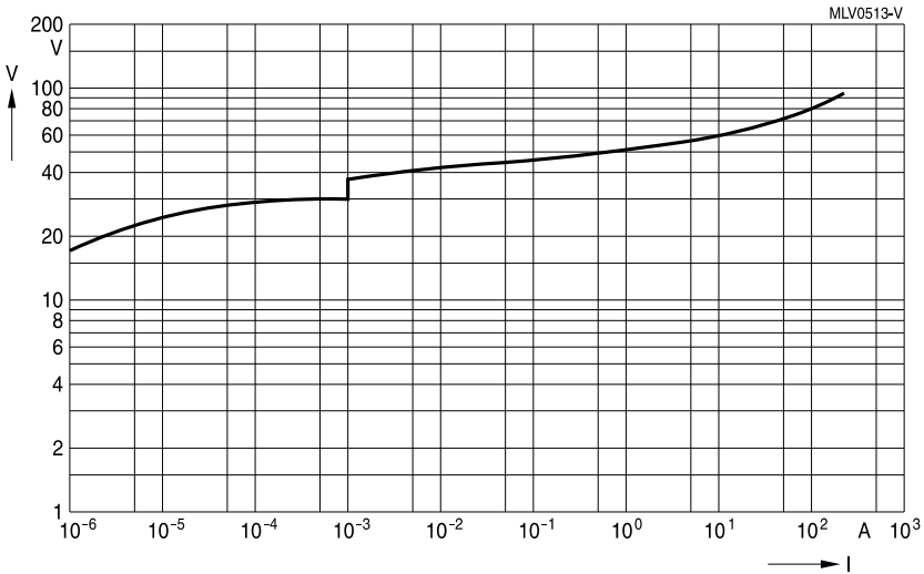
CT1210K20AUTOG
