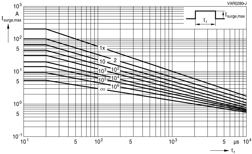
CT1206K14G ... K30G
