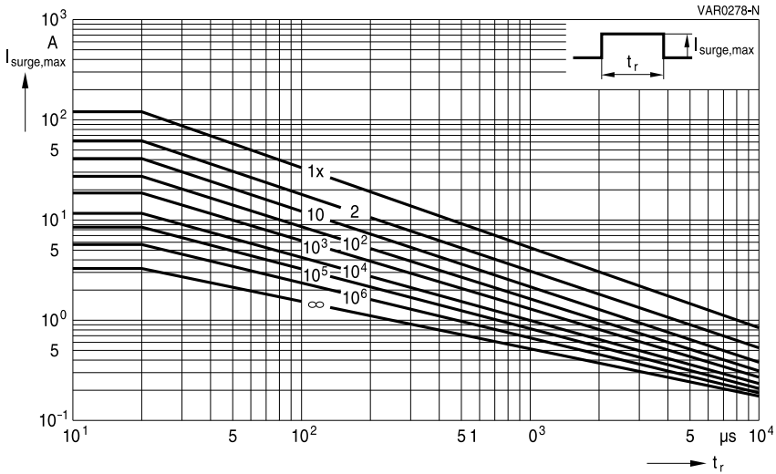
CT0805K11G ... K17G
