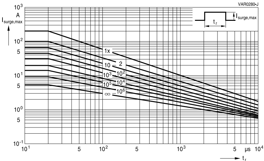
CT1206K20AUTOG
