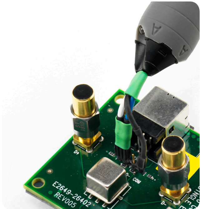
Figure 5 With the N4822A socketed tip (optional)
