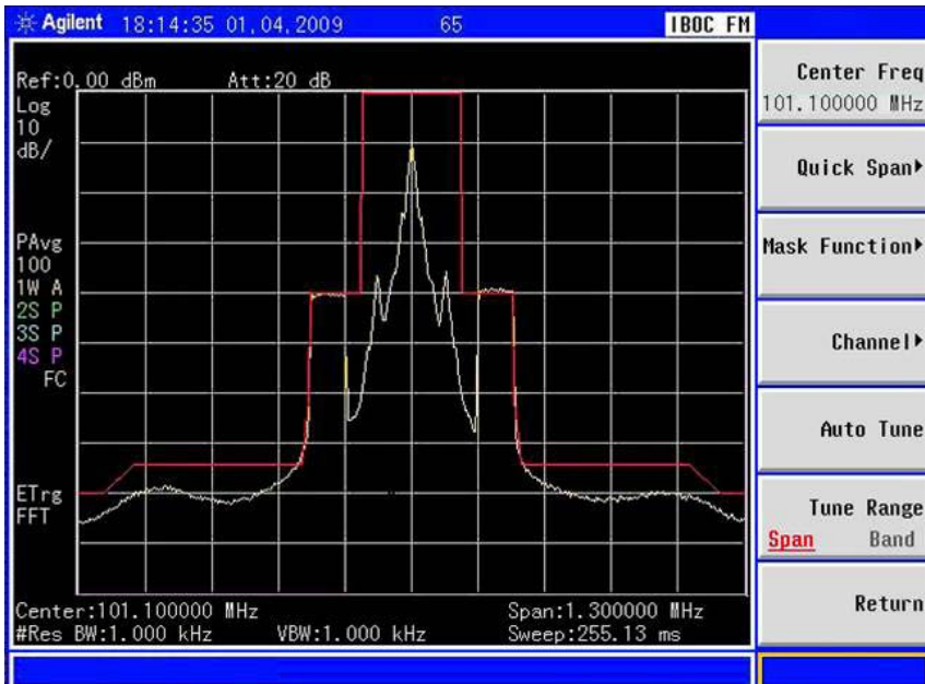
IBOC-FM measurement with N9340B IBC
