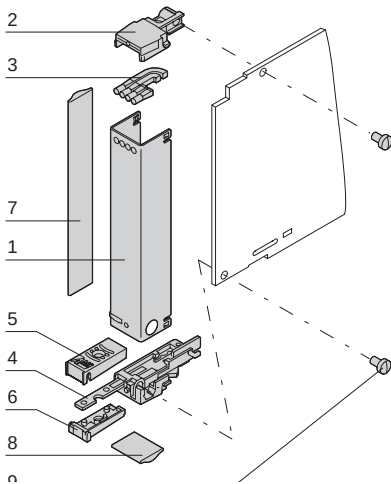
Single AdvancedMC modules
