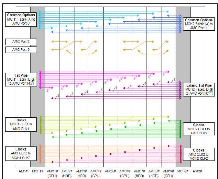
Backplane topology
