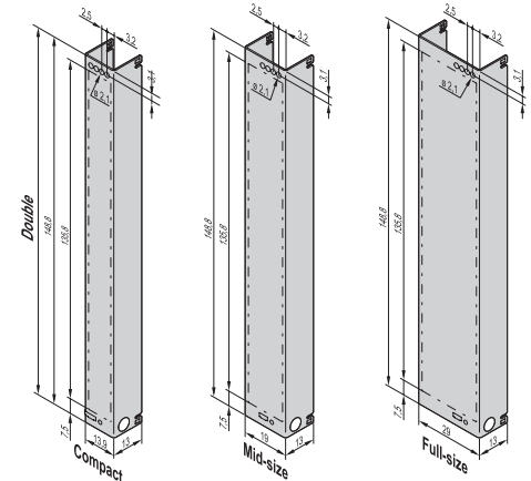
Double AdvancedMC modules
