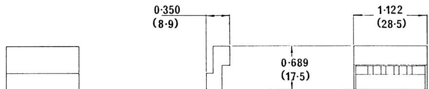
Pattern C for Use on Bobbin Size 18 (S08000/GNN/BLK)
