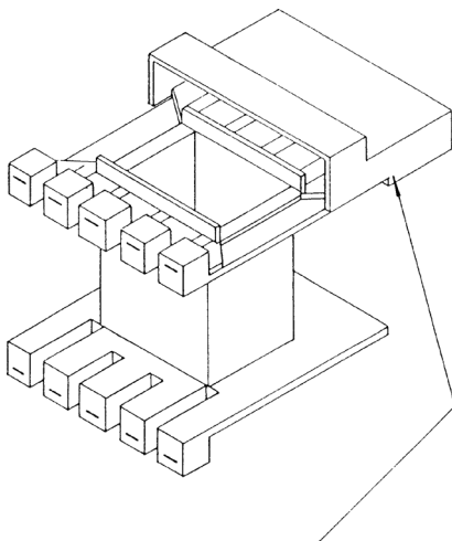
Insulator Fitted to One Bobbin Cheek
