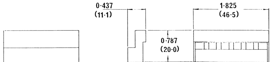
Pattern A for Use on Bobbin Sizes 29 and 196 (S07900/GNN/BLK)
