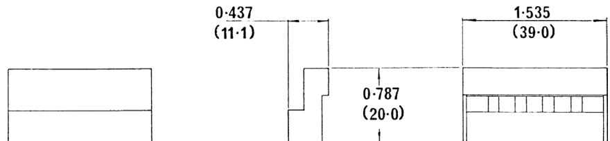
Pattern B for Use on Bobbin Sizes 35 and 147 (S07800/GNN/BLK)
