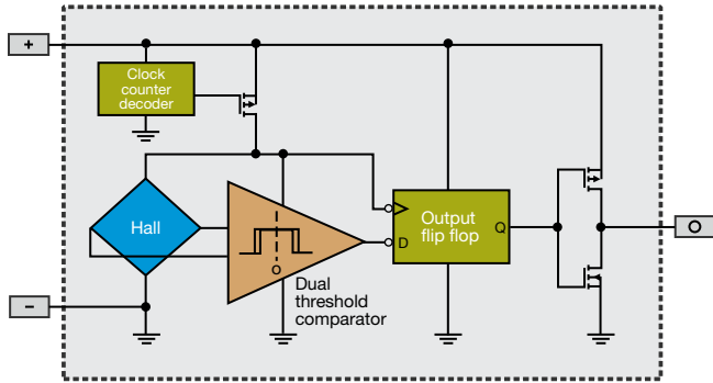
Figure 1. Block/Electric Diagram
