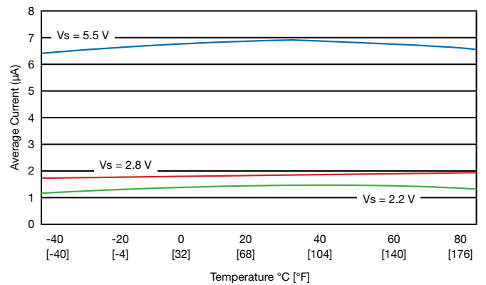
Figure 6. Typical Average Current vs Temperature
