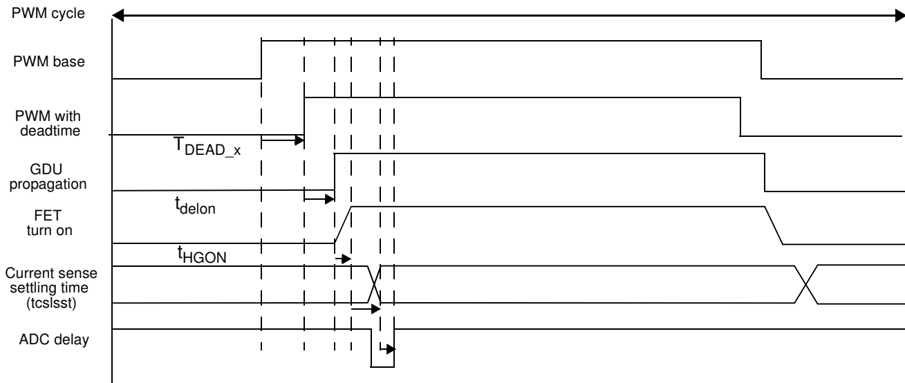
Figure 1-8. Control Loop Delay Overview
