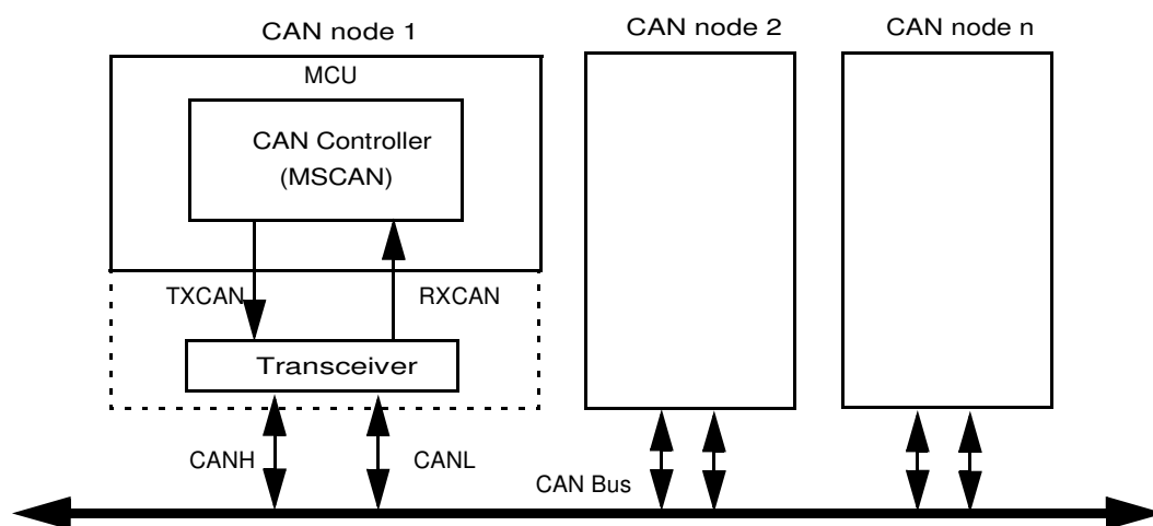
Figure 12-2. CAN System
