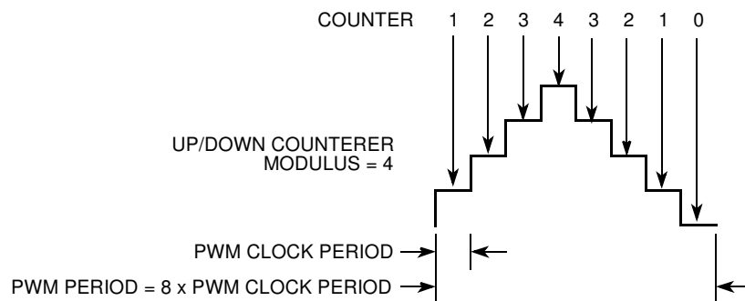
Figure 14-44. Center-Aligned PWM Period
