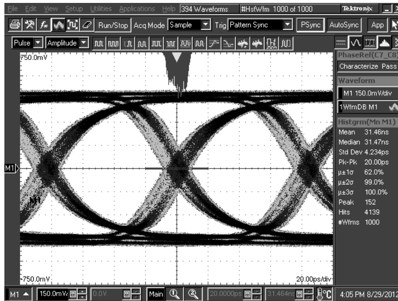
DS125BR401 settings: EQ[1:0] = R, 0 = 07'h, DEM[1:0] = 0, 1 Figure 20. TL1 = 5-meter 30-AWG 100 Ohm Twin-axial Cable, 12 Gbps
