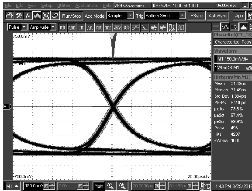
DS125BR401 settings: EQ[1:0] = 0, 1 = 03'h, DEM[1:0] = 0, 1 Figure 15. TL = 20 inch 5-mil FR4 trace, 8 Gbps
