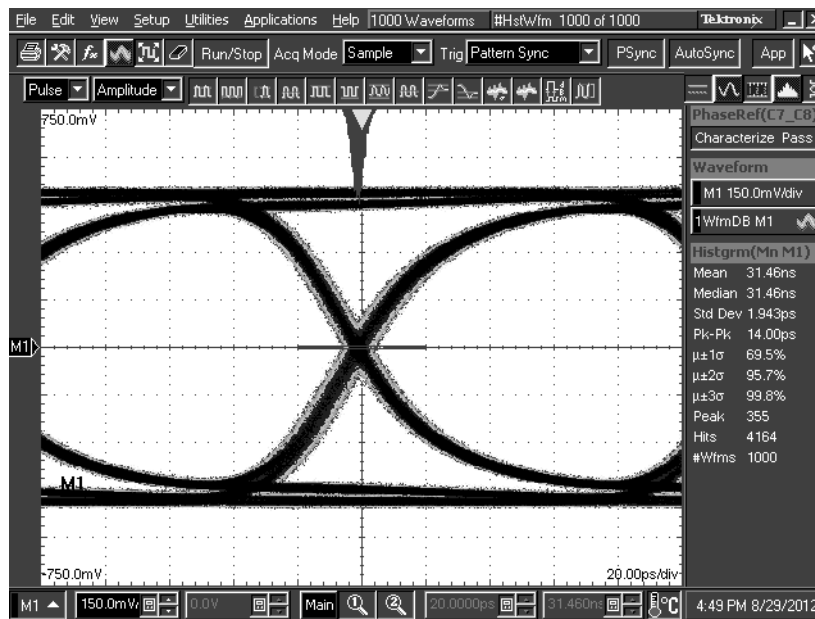
DS125BR401 settings: EQ[1:0] = R, 0 = 07'h, DEM[1:0] = 0, 1 Figure 18. TL = 30 inch 5-mil FR4 trace, 8 Gbps
