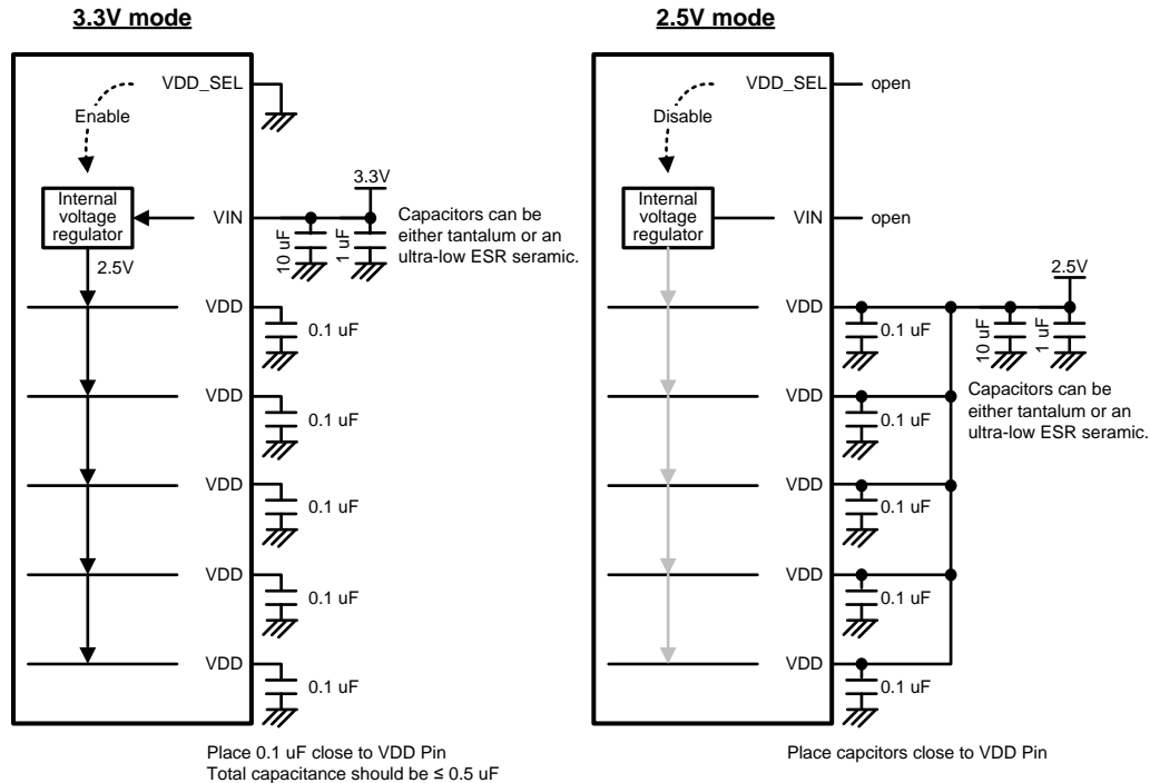
Figure 5. 3.3V or 2.5V Supply Connection Diagram
