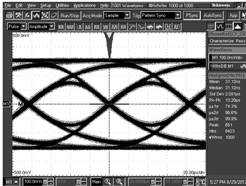
DS125BR401 settings: EQ[1:0] = R, 1 = 0F'h, DEM[1:0] = R, 0 Figure 25. TL1 = 20 inch 5-mil FR4 trace, TL2 = 10 inch 5-mil FR4 trace, 12 Gbps
