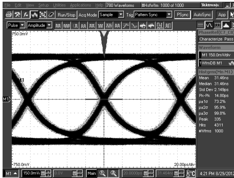
DS125BR401 settings: EQ[1:0] = R, 0 = 07'h, DEM[1:0] = 0, 1 Figure 19. TL = 30 inch 5-mil FR4 trace, 12 Gbps
