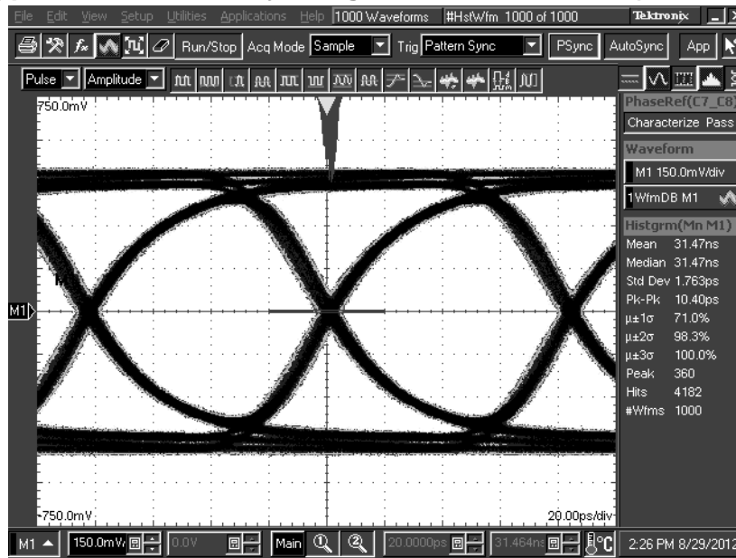
DS125BR401 settings: EQ[1:0] = 0, R = 01'h, DEM[1:0] = 0, 1 Figure 13. TL = 10 inch 5-mil FR4 trace, 12 Gbps
