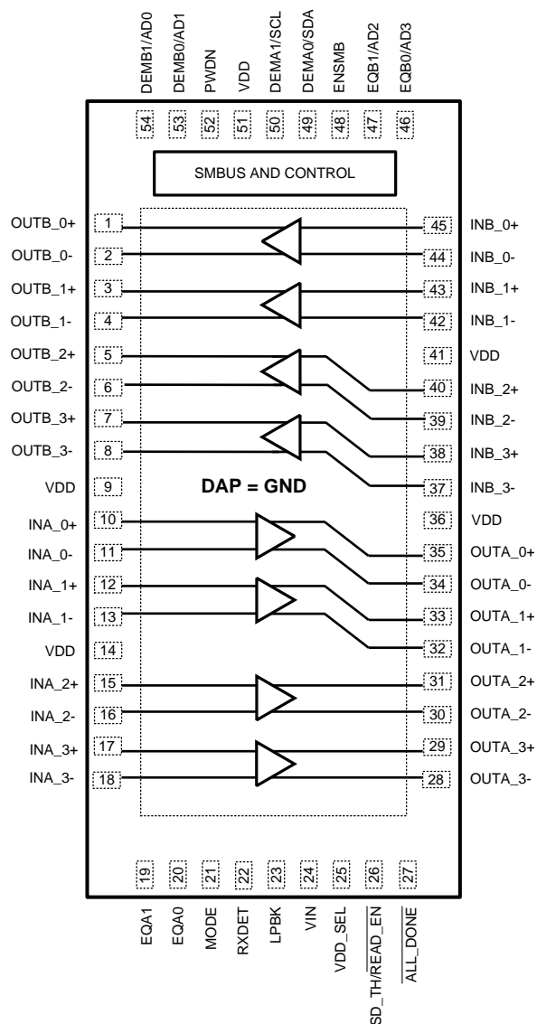
DS125BR401 Pin Diagram 54-lead WQFN Package See Package Number NJY0054A
