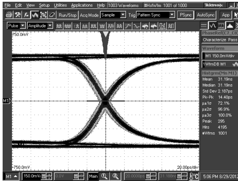
DS125BR401 settings: EQ[1:0] = R, 0 = 07'h, DEM[1:0] = 0, 1 Figure 17. TL = 30 inch 5-mil FR4 trace, 5 Gbps
