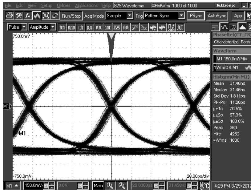
DS125BR401 settings: EQ[1:0] = 0, 1 = 03'h, DEM[1:0] = 0, 1 Figure 16. TL = 20 inch 5-mil FR4 trace, 12 Gbps
