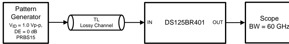
Figure 10. Test Setup Connections Diagram
