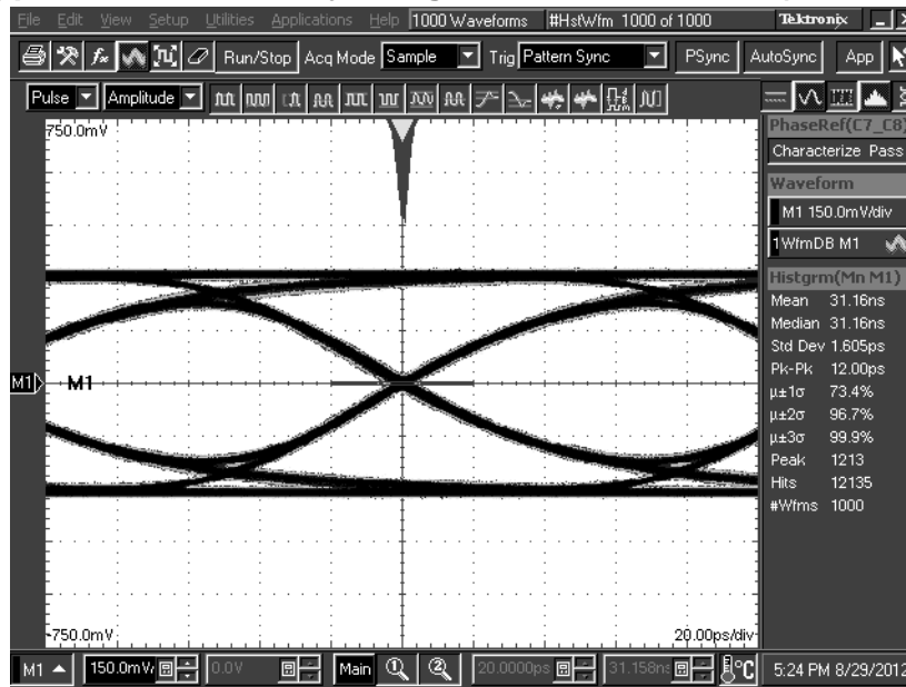
DS125BR401 settings: EQ[1:0] = R, 1 = 0F'h, DEM[1:0] = R, 0 Figure 24. TL1 = 20 inch 5-mil FR4 trace, TL2 = 10 inch 5-mil FR4 trace, 8 Gbps
