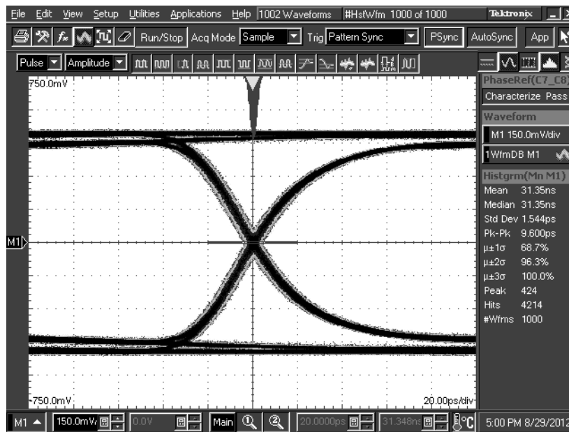
DS125BR401 settings: EQ[1:0] = 0, 1 = 03'h, DEM[1:0] = 0, 1 Figure 14. TL = 20 inch 5-mil FR4 trace, 5 Gbps
