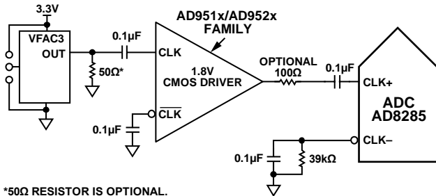
Figure 30. Single-Ended 1.8 V CMOS Sample Clock
