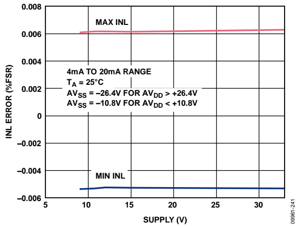
Figure 42. Integral Nonlinearity Error vs. Supply, Internal R SET
