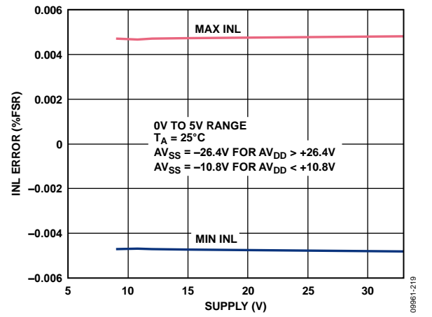
Figure 20. Integral Nonlinearity Error vs. Supply
