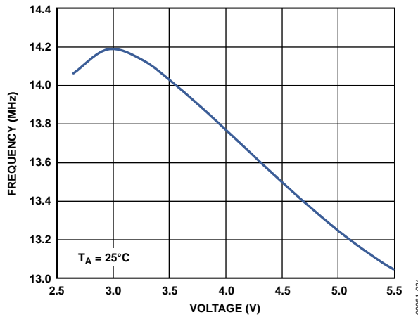
Figure 69. Internal Oscillator Frequency vs. DV DD Supply Voltage
