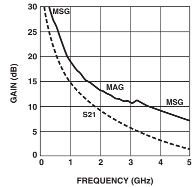
Figure 20. AT-41511 Gains vs. Frequency at V_{CE} = 8V , I_C = 25 \text{ mA} .
