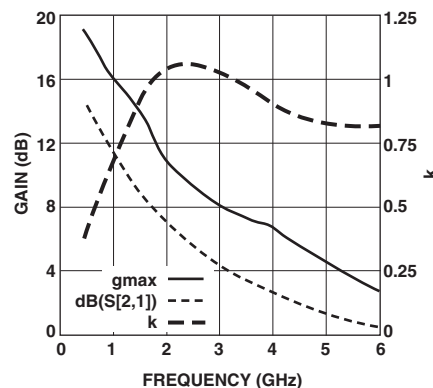
Figure 10. Gain vs. Frequency at 2.7 V, 2 mA.
