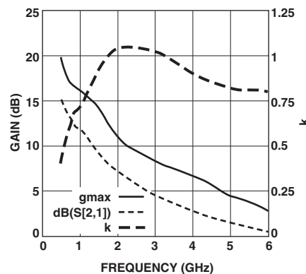
Figure 13. Gain vs. Frequency at 5 V, 2 mA.
