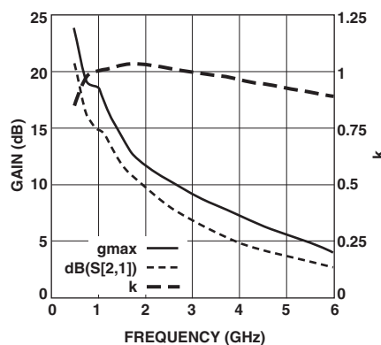
Figure 15. Gain vs. Frequency at 5 V, 10 mA.
