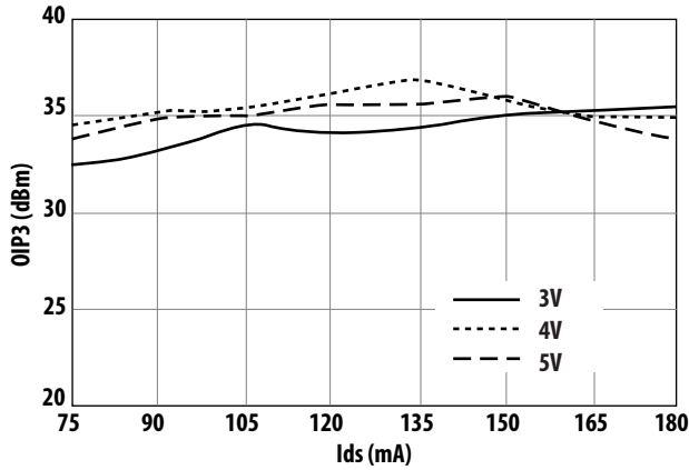
Figure 13. OIP3 vs. Ids and Vds at 5.8 GHz
