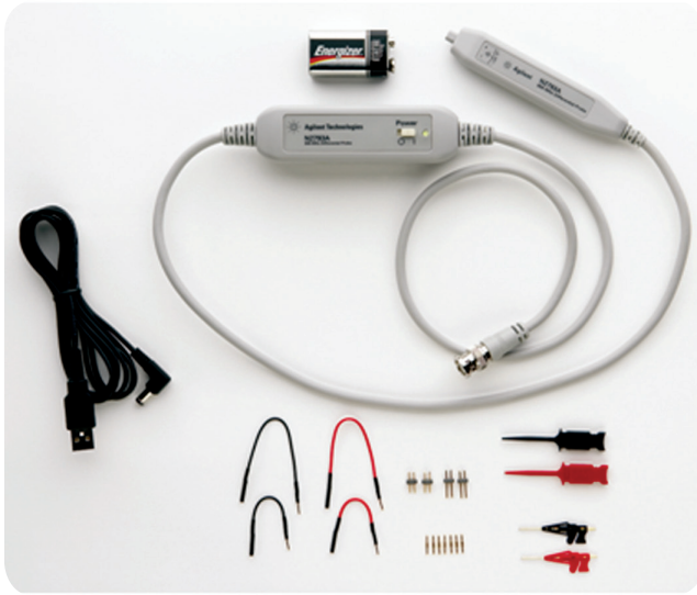
Figure 8. N2793A 800 MHz differential probe with standard accessories
