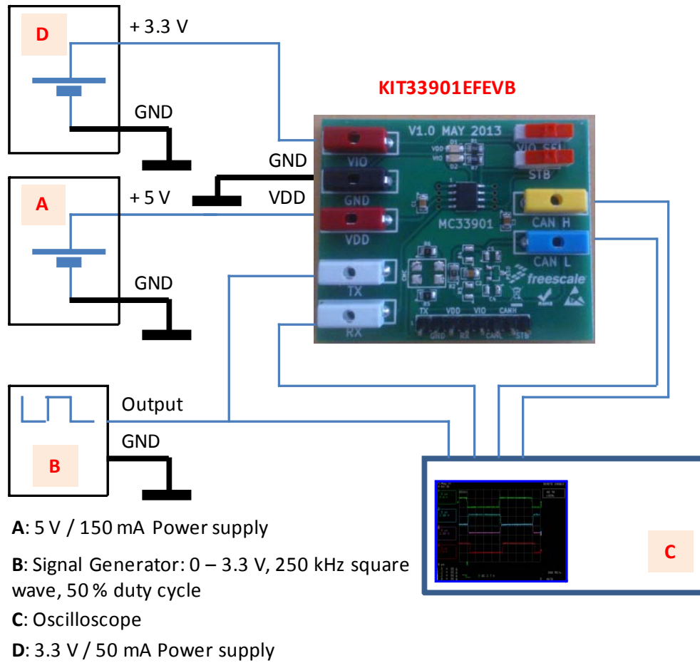
Figure 4. KIT33901EFEVB Board Setup with Dual Power Supply
