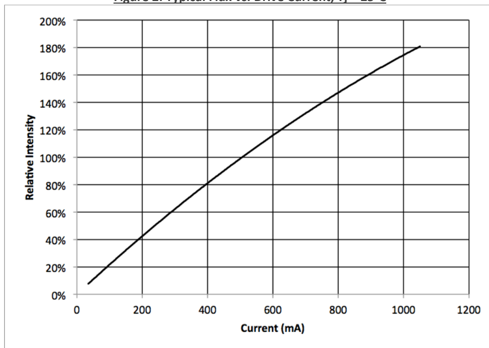
Figure 2: Typical Flux vs. Drive Current, T j = 25°C
