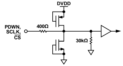
Figure 38. Equivalent PDWN, SCLK, or \overline{CS} Input Circuit
