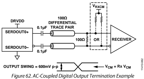
Figure 62. AC-Coupled Digital Output Termination Example
