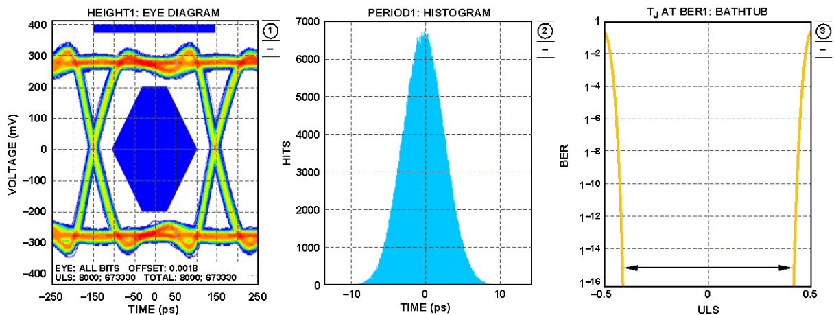
Figure 65. AD9683 Digital Outputs Data Eye, Histogram and Bathtub, External 100 \Omega Terminations at 3.4 Gbps
