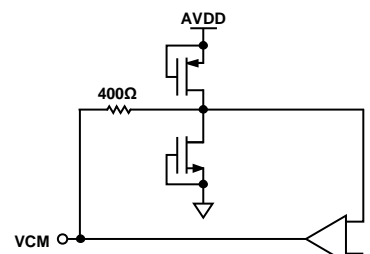
Figure 42. Equivalent VCM Circuit
