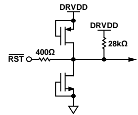
Figure 41. Equivalent \overline{RST} Input Circuit
