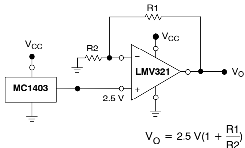
Figure 28. Voltage Reference
