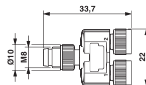
Dimensioned drawing
