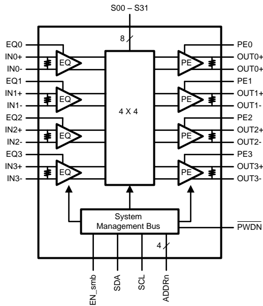
DS25CP104A
