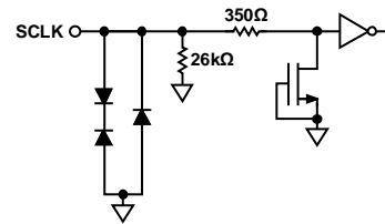
Figure 44. Equivalent SCLK Input Circuit
