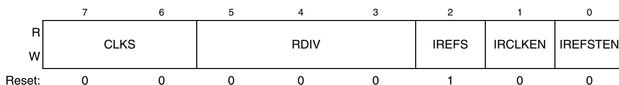
Figure 12-3. MCG Control Register 1 (MCGC1)
