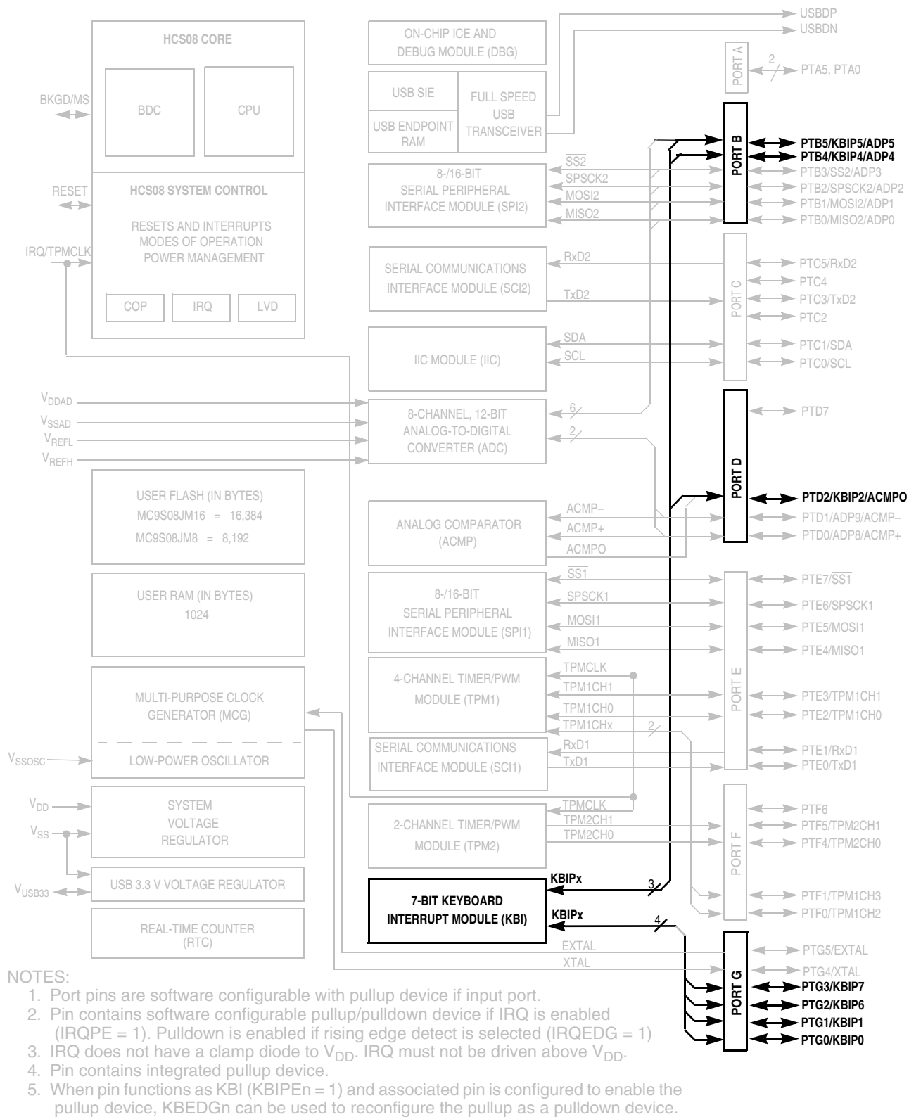
Figure 8-1. MC9S08JM16 Series Block Diagram Highlighting KBI Block and Pins
