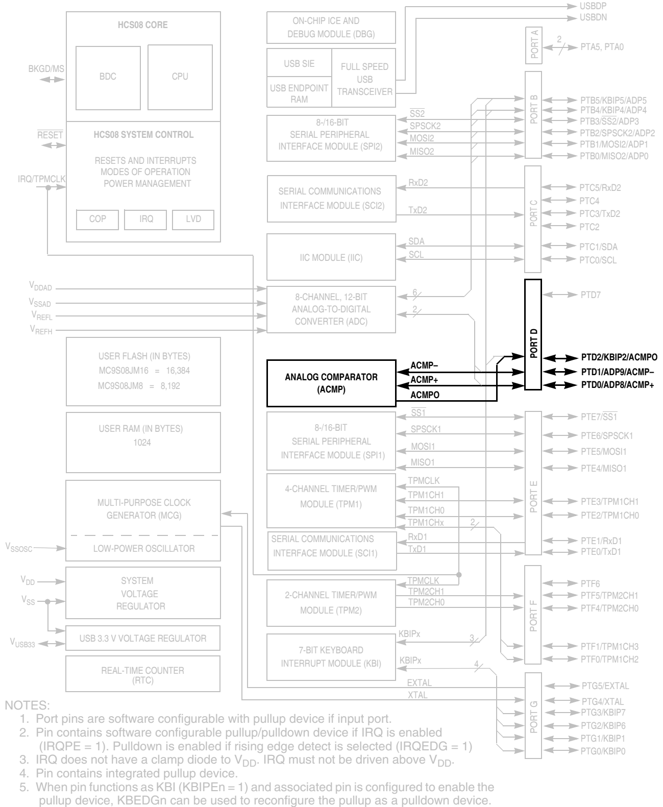
Figure 9-1. MC9S08JM16 Series Block Diagram Highlighting ACMP Block and Pins
