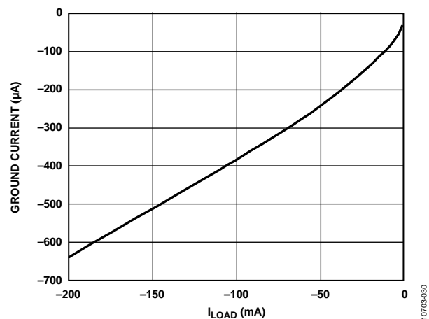
Figure 32. Ground Current vs. Load Current ( I_{LOAD} ), V_{OUT} = -1.8 V
