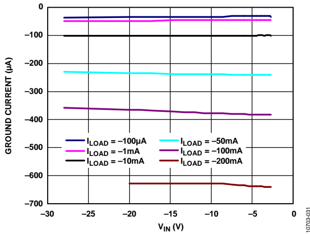
Figure 33. Ground Current vs. Input Voltage ( V_{IN} ), V_{OUT} = -1.8 V
