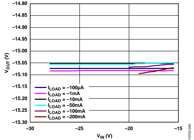
Figure 42. Output Voltage ( V_{OUT} ) vs. Input Voltage ( V_{IN} ), Adjustable Output Voltage, V_{OUT} = -15 V
