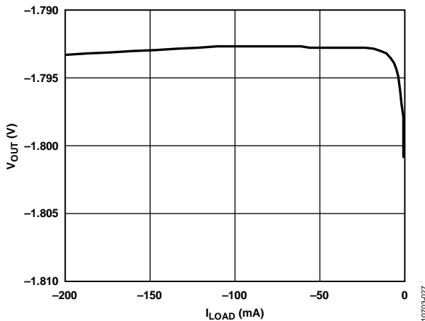
Figure 29. Output Voltage ( V_{OUT} ) vs. Load Current ( I_{LOAD} ), V_{OUT} = -1.8 V
