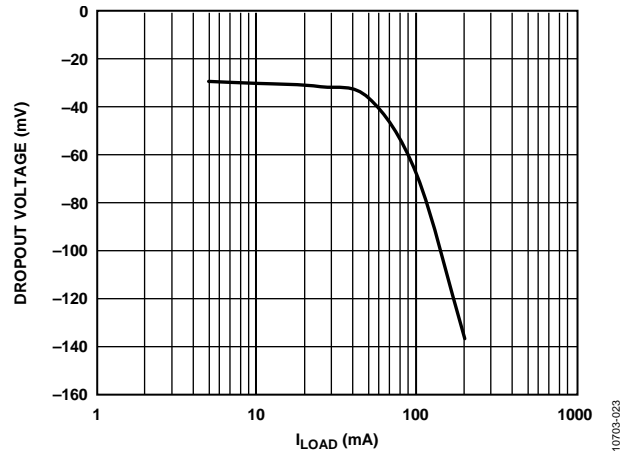
Figure 25. Dropout Voltage vs. Load Current ( I_{LOAD} ), V_{OUT} = -5 V
