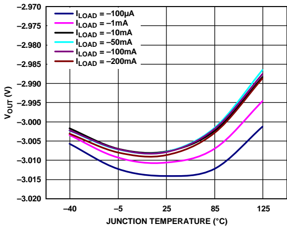
Figure 9. Output Voltage ( V_{OUT} ) vs. Junction Temperature ( T_j )
