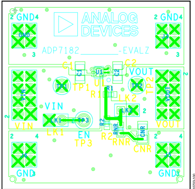
Figure 101. Example of the 6-Lead LFCSP PCB Layout
