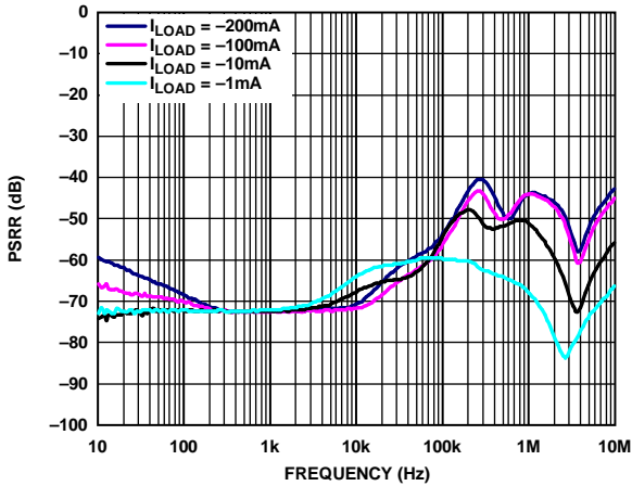
Figure 53. Power Supply Rejection Ratio (PSRR) vs. Frequency, V_{OUT} = -1.8\text{ V} vs. Different Load Currents ( I_{LOAD} ), V_{IN} = -5.5\text{ V}
