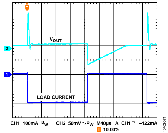
Figure 76. Load Transient Response, V_{OUT} = -15\text{ V} , I_{LOAD} = -1\text{ mA} to -200\text{ mA} , Load Step = 1\text{ A}/\mu\text{s} , Noise Reduction Network
