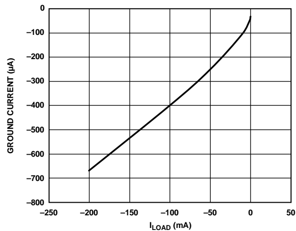
Figure 13. Ground Current vs. Load Current ( I_{LOAD} )
