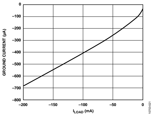
Figure 23. Ground Current vs. Load Current ( I_{LOAD} ), V_{OUT} = -5 V
