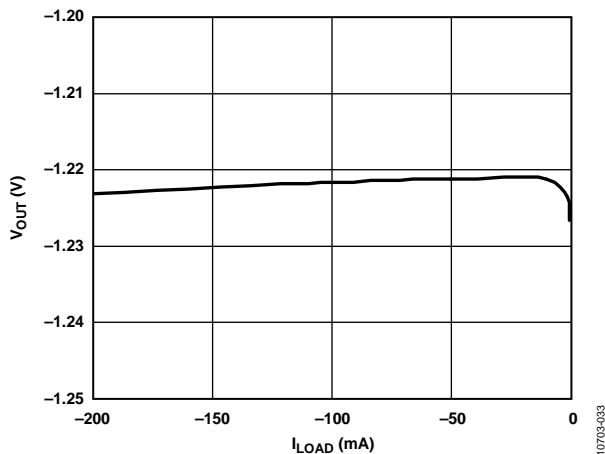
Figure 35. Output Voltage ( V_{OUT} ) vs. Load Current ( I_{LOAD} ), V_{OUT} = -1.22 V
