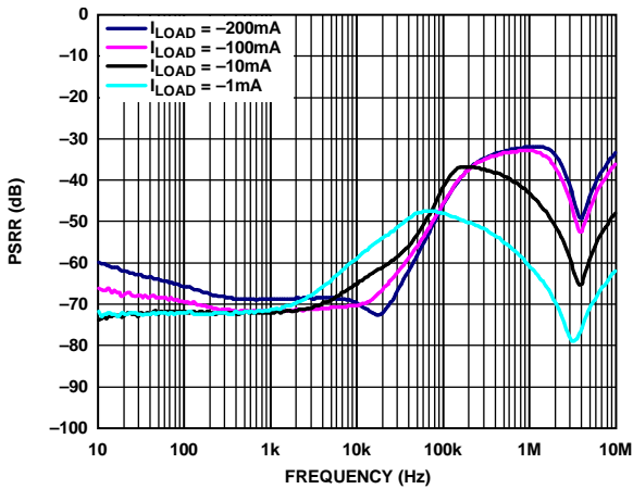
Figure 52. Power Supply Rejection Ratio (PSRR) vs. Frequency, V_{OUT} = -1.8\text{ V} vs. Different Load Currents ( I_{LOAD} ), V_{IN} = -2.8\text{ V}
