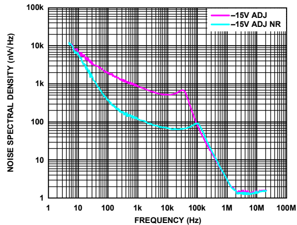
Figure 88. –15 V Adjustable ADP7182 with and without the Noise Reduction Network ( C_{NR} and R_{NR} )
