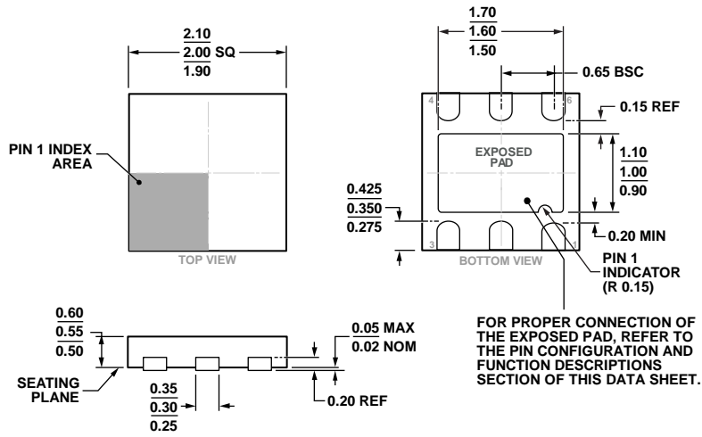
Figure 104. 6-Lead Lead Frame Chip Scale Package [LFCSP_UD] 2.00 mm x 2.00 mm Body, Ultra Thin, Dual Lead (CP-6-3) Dimensions shown in millimeters
