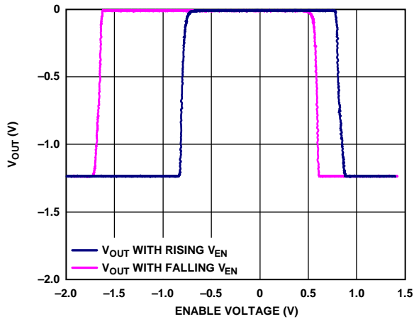
Figure 82. Typical EN Pin Operation
