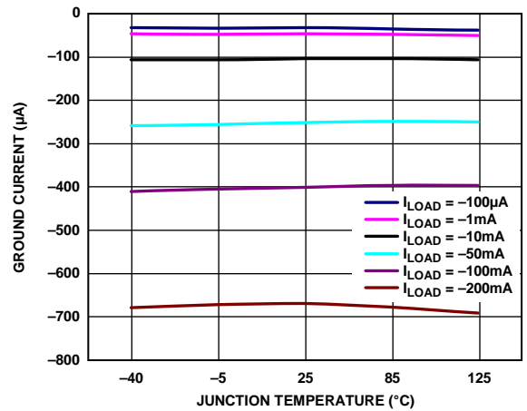
Figure 12. Ground Current vs. Junction Temperature ( T_j )
