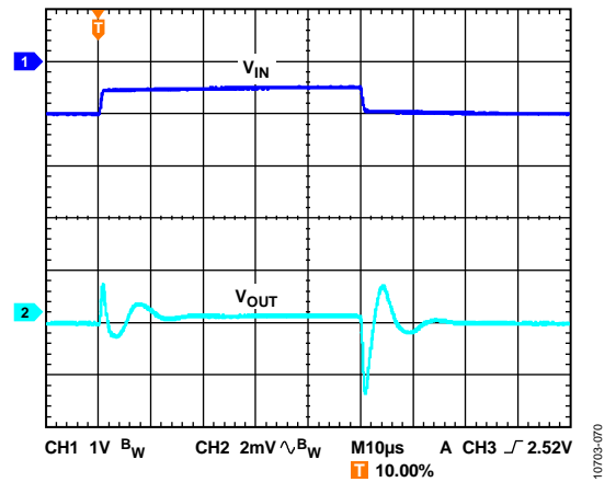
Figure 72. Line Transient Response, 500 mV Step, V_{OUT} = -15\text{ V} , Noise Reduction Network, I_{LOAD} = -10\text{ mA}
