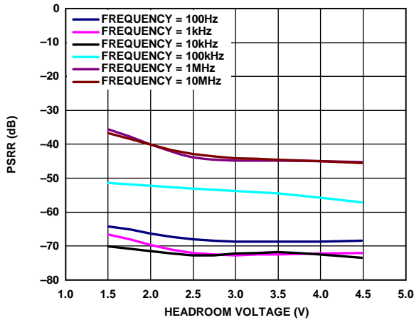
Figure 51. Power Supply Rejection Ratio (PSRR) vs. Headroom Voltage, V_{OUT} = -1.22\text{ V} , Load Current ( I_{LOAD} ) = -200\text{ mA}
