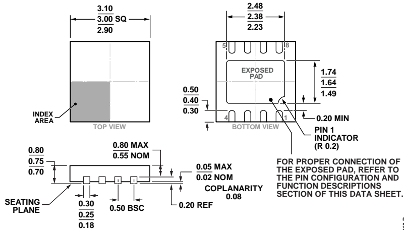
COMPLIANT TO JEDEC STANDARDS MO-229-WEED-4 Figure 105. 8-Lead Lead Frame Chip Scale Package [LFCSP_WD] 3 mm x 3 mm Body, Very Very Thin, Dual Lead (CP-8-5) Dimensions shown in millimeters
