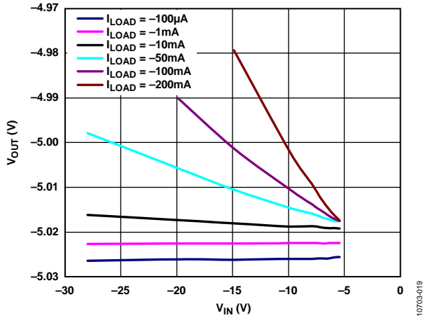
Figure 21. Output Voltage vs. Input Voltage ( V_{IN} ), V_{OUT} = -5 V
