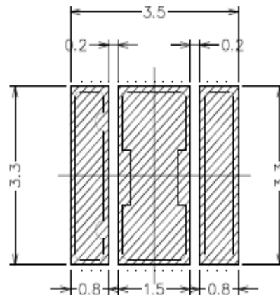
Soldering patterns
