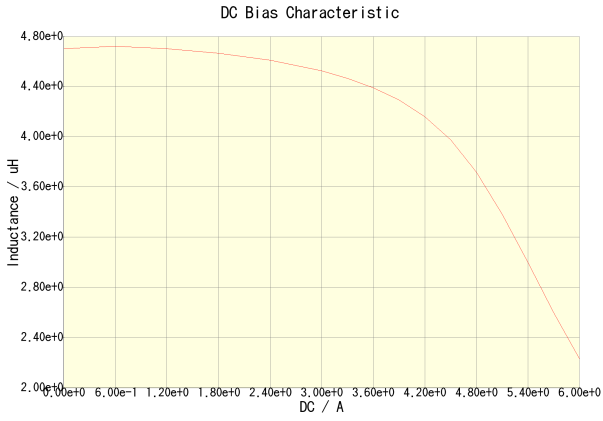
SLF7045T-4R7M2R1-H(Amb. Temp. = 20degc)
