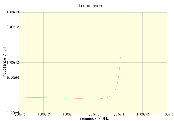
SLF12565T-220M3R5-H
