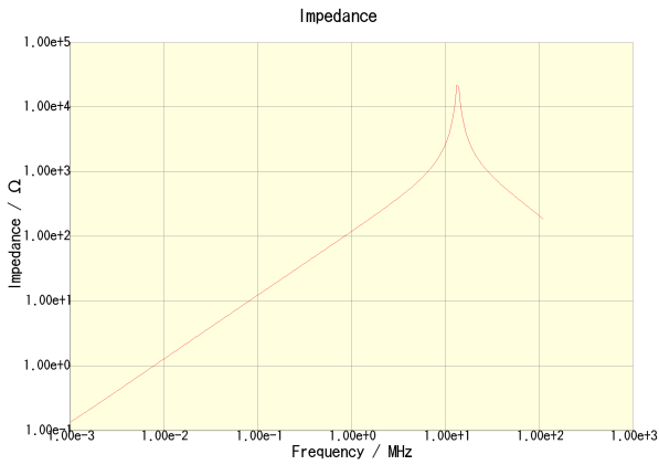
SLF12565T-220M3R5-H
