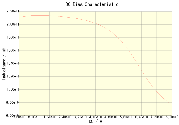
SLF12565T-220M3R5-H(Amb. Temp. = 20degc)
