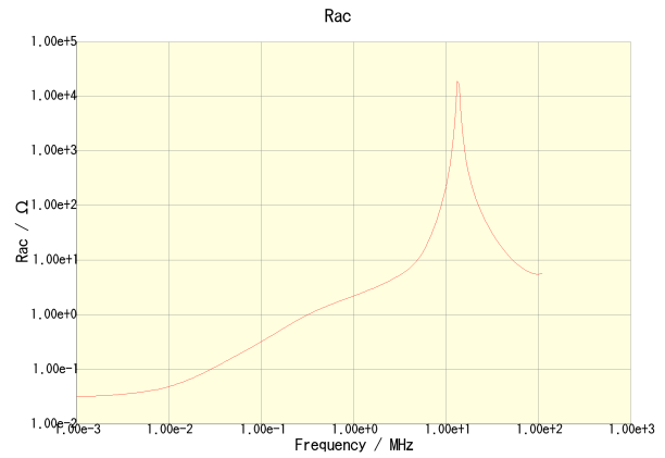
SLF12565T-220M3R5-H
