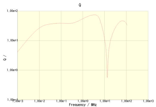
SLF12565T-220M3R5-H
