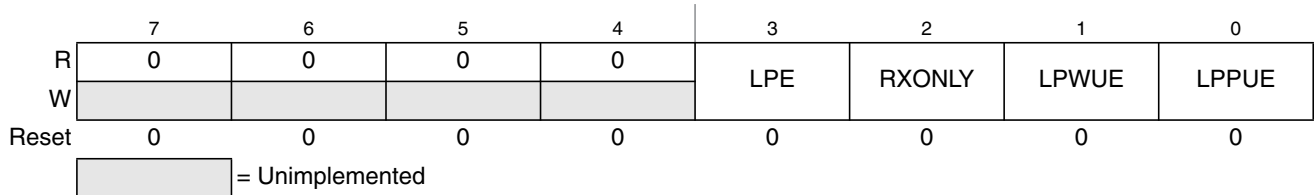
Figure 15-4. LIN Control Register (LPCR)
