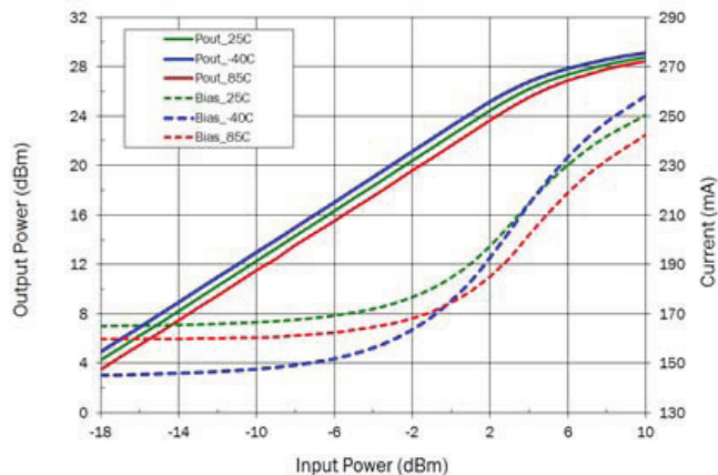
Output Power and Icc versus Input Power at 880MHz
