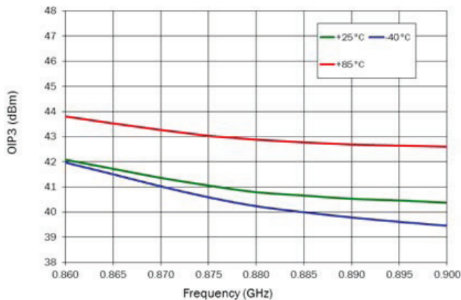
OIP3 versus Frequency (15dBm tones)
