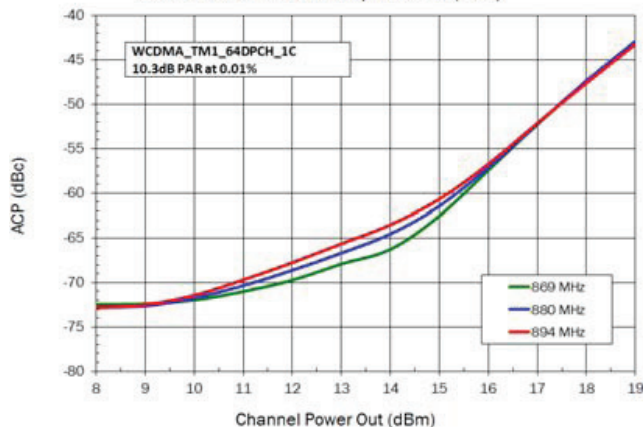
ACPR versus WCDMA Output Power (25C)
