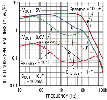
Output Noise Spectral Density vs C_{REF/BYP} = 0, C_{FF} = 0
