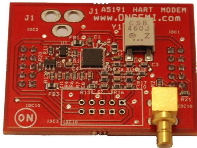
Figure 1. A5191HRTNGEVB Evaluation Board
